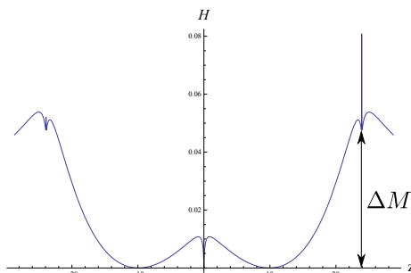
Figure 8. The metastable supertube brings in an excess energy \Delta M = M_{ADM}^{\text{BH}} - \sum_I Q_I^{\text{BH}} .
