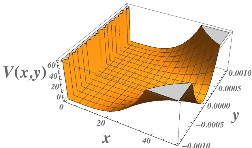
Figure 1. The potential V(x,y) for a = b = \alpha = 1 in no-scale supergravity with the stabilized Kähler potential (2.21) and the superpotential (2.19).
