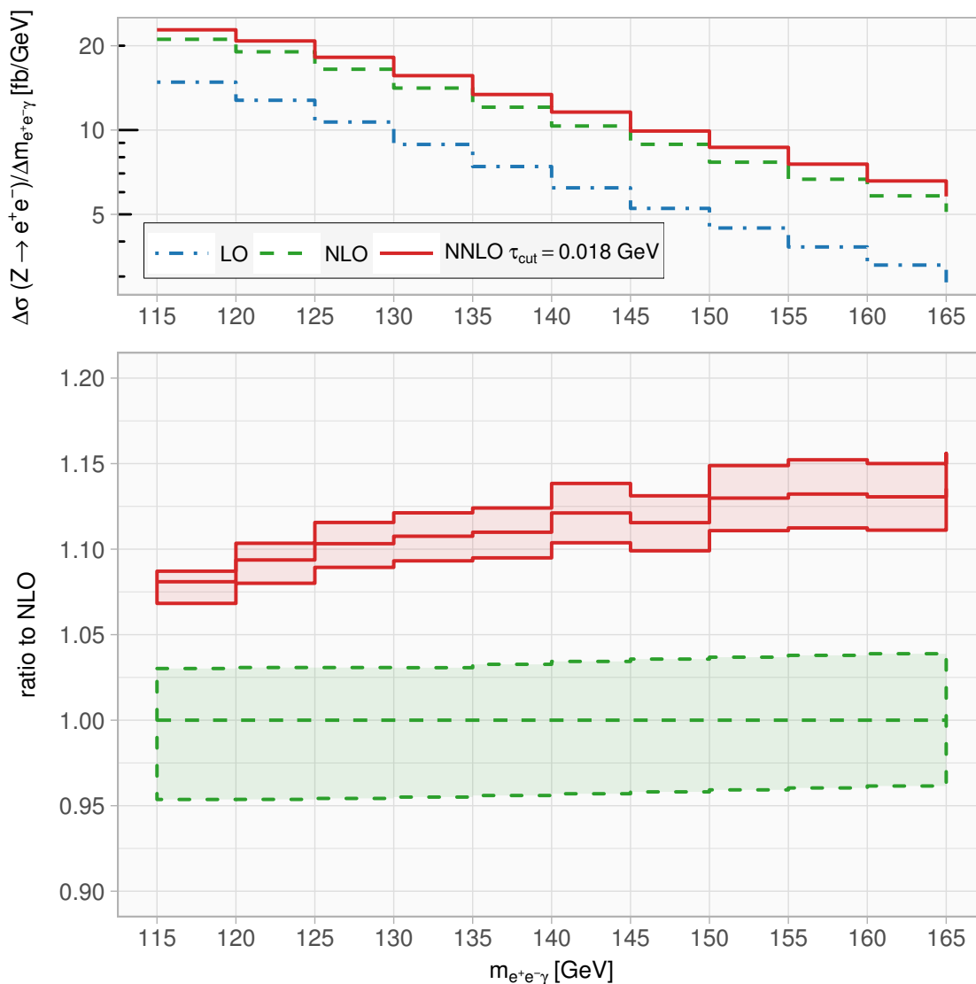
Figure 11. Invariant mass distribution m_{e^+e^- \gamma} of the e^+e^- \gamma system for the electron decay channel with cuts in table 5. In the upper panel the absolute distribution is shown, whereas in the lower panel the ratio to the NLO result is displayed. The reported numerical integration uncertainty is about 0.2% for the NNLO results.
