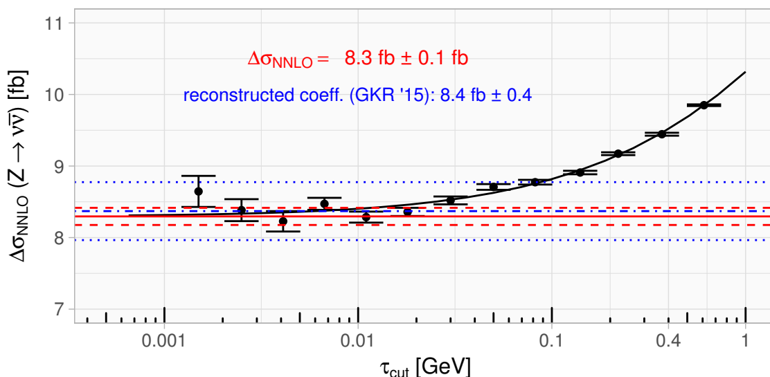
Figure 4. \tau_{\text{cut}} dependence of NNLO cross section coefficient in the neutrino decay channel with given cuts in table 2 . The horizontal red solid and dashed lines represent the fitted asymptotic value of 8.3(1)fb and its numerical uncertainty, respectively, while the solid black line shows the fitted result. The blue dot-dashed and dotted lines show the reconstructed NNLO coefficient and its numerical uncertainty, respectively, from the NNLO result given in ref. [39].
