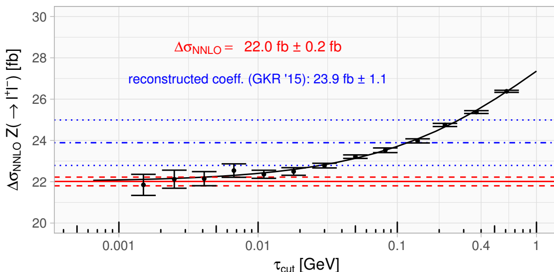
Figure 5. \tau_{\text{cut}} dependence of the NNLO cross section coefficient in the charged lepton decay channel with cuts given in table 1. The horizontal red solid and dashed lines represent the fitted asymptotic value of 22.0(2)fb and its numerical uncertainty, respectively, while the solid black line shows the fitted result. The blue dot-dashed and dotted lines show the reconstructed NNLO coefficient and its numerical uncertainty, respectively, from the NNLO result given in ref. [39].
