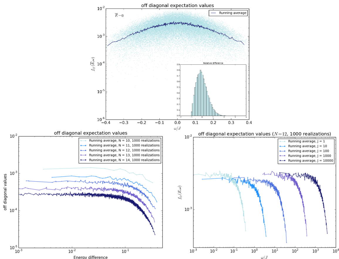
Figure 3. Off-diagonal values of matrix elements \mathcal{O}_{nm} = |\langle n|\mathcal{O}|m\rangle| for the single-site number operator \mathcal{O} = \hat{n}_N at half filling \nu = \frac{1}{2} . We show the off-diagonal matrix elements against their energies E_n/J . Top panel: N = 14 with raw data in light blue and the running average in dark blue. The inset shows a histogram of relative error between raw data and running average. We see that the histogram is peaked around zero. Left panel: the function f_{\mathcal{O}}(\bar{E}, \omega) (we show the running average) for varying Hilbert space dimension corresponding to N = 10, 11, 12, 13, 14 . The cross-over from constant to non-constant behavior is identified with the Thouless energy E_T . Right panel: scaling of the Thouless energy with average coupling strength J . A simple fit gives E_T \propto J^2 .
