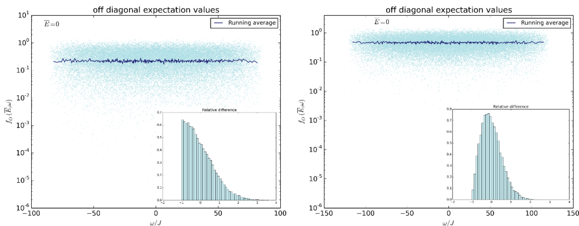
Figure 10. Off-diagonal values of matrix elements O_{nm} = |\langle n|\mathcal{O}|m\rangle| for a randomly chosen operator \mathcal{O} in random matrix theory (a GOE matrix on the left and a GUE matrix on the right) averaged over 1000 realizations. The inset shows a histogram of relative differences between raw data and running average (within a selected energy window). Left panel: the function f_{\mathcal{O}}(\bar{E}, \omega) (we show the running average in dark blue and the raw data in light blue) in the GOE for Hilbert space dimension \dim(\mathcal{H}) = 2^{12} . One clearly sees the constancy of f_{\mathcal{O}}(\bar{E}, \omega) in RMT. Right panel: the function f_{\mathcal{O}}(\bar{E}, \omega) (we show the running average in dark blue and the raw data in light blue) in the GUE for Hilbert space dimension \dim(\mathcal{H}) = 2^{12} . One clearly sees the constancy of f_{\mathcal{O}}(\bar{E}, \omega) in RMT.
