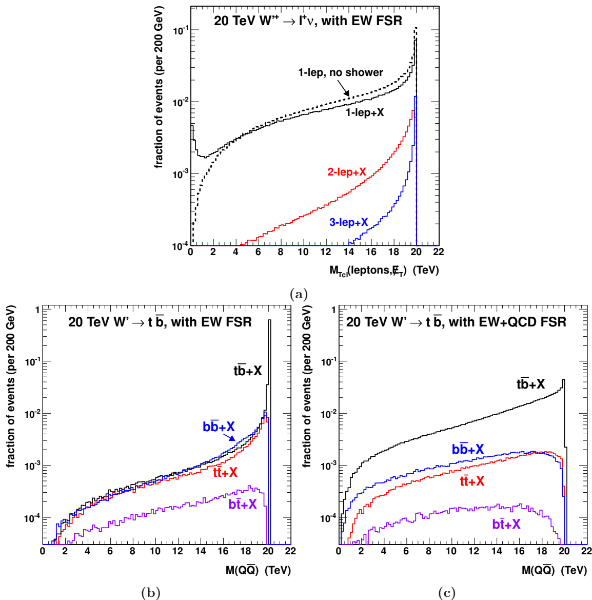
Figure 10. Showered events from 20 TeV W'^+ decays. (a) W'^+ \rightarrow \nu_L \ell_R^+ cluster transverse mass distributions, running the full EW shower and breaking down the signal by inclusive lepton multiplicity (solid curves), as well as the uncorrected two-body decay result (dotted curve). (b) W'^+ \rightarrow t_L \bar{b}_R quark-pair invariant mass distributions, running the full EW shower, and (c) combining EW and QCD showering.
