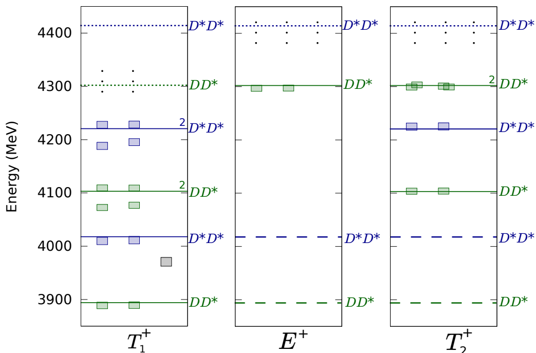
Figure 6. As figure 5 but for the isospin-0 doubly-charmed sector with quark flavour ccl\bar{l} . Dashed lines indicate kinematic thresholds where a non-interacting level is not expected. Dotted lines indicate non-interacting meson-meson levels where the corresponding operators have not been included in the operator basis. Ellipses indicate that additional energy levels have been extracted in/above these regions but we have not plotted them as we have not included all relevant meson-meson operators in these energy regions.
