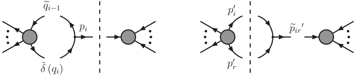
Figure 2. Factorization of the dual one-loop and tree-level squared amplitudes in the collinear limit. The dashed line represents the momentum conservation cut.
