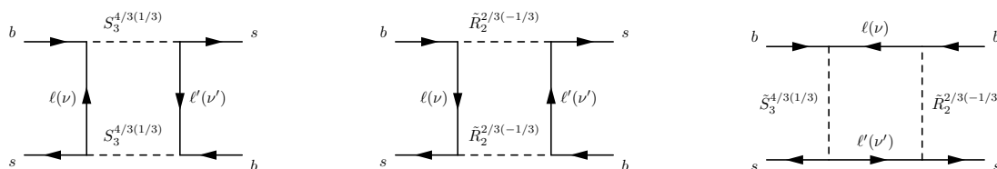
Figure 1. Three types of box-diagrams with S_3 and \tilde{R}_2 contributing to \Delta m_s .
