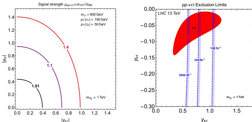
Figure 6. (Left panel) Contours of constant signal strength \mu_{pp \rightarrow \tau\tau} for different deviations from the SM prediction at m_{S_3} = 1 TeV. (Right panel) 95% C.L. limits for LHC luminosities of 100, 300, and, 3000 \text{fb}^{-1} (dotted blue contours) from recasting high-mass \tau\tau searches by ATLAS [83] for m_{S_3} = 1 TeV. The red region corresponds to the 1\sigma low-energy fit.
