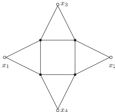
Figure 1. A four-loop conformal integral.
