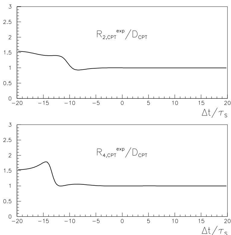
Figure 1. The ratios R_{2,\text{CPT}}^{\text{exp}}(\Delta t) and R_{4,\text{CPT}}^{\text{exp}}(\Delta t) as a function of \Delta t . For visualization purposes the CPT violating parameters have been fixed to the values \Re\delta = 3.3 \times 10^{-4} and \Im\delta = 1.6 \times 10^{-5} .
