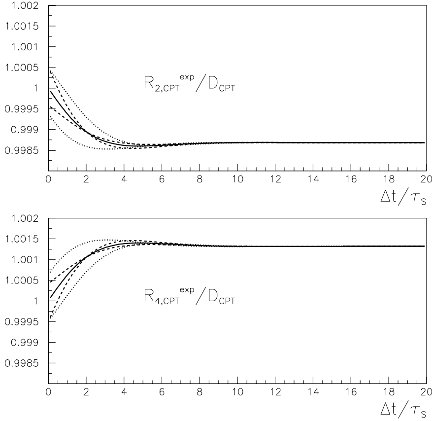
Figure 4. A zoom of the plots shown in figure 3 in the region 0 \leq \Delta t \leq 20\tau_S .
