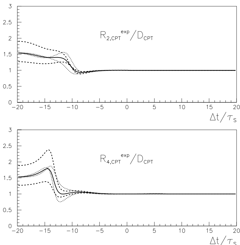
Figure 3. The expected ratios for the CPT test R_{2,\text{CPT}}^{\text{exp}}(\Delta t) (top) and R_{4,\text{CPT}}^{\text{exp}}(\Delta t) (bottom) as a function of \Delta t (solid line); dashed lines correspond to \pm 10\% variation in the absolute value of \eta_{3\pi^0} , while dotted lines correspond to a \pm 10^\circ variation of its phase (with respect to the value \eta_{3\pi^0} = \epsilon_S ). For visualization purposes the CPT violating parameters have been fixed to the values \Re\delta = 3.3 \times 10^{-4} and \Im\delta = 1.6 \times 10^{-5} .
