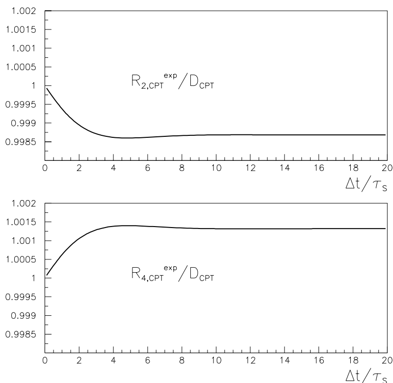
Figure 2. A zoom of the plots shown in figure 1 in the region 0 \leq \Delta t \leq 20\tau_S .
