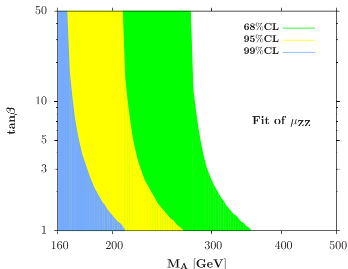
Figure 6. The [\tan\beta, M_A] parameter space of the MSSM in which the signal strength in the h \rightarrow ZZ search channel is not compatible with the LHC data on the rates of the observed h boson at the 68%CL (green), 95%CL (yellow) and 99%CL (blue).
