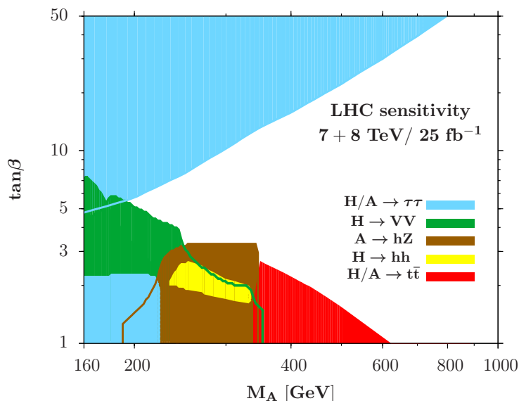
Figure 10. The estimated sensitivities in the various search channels for the heavier MSSM Higgs bosons in the [\tan\beta, M_A] plane: H/A \rightarrow \tau^+\tau^- (light blue), H \rightarrow WW + ZZ (green), H/A \rightarrow t\bar{t} (red), A \rightarrow hZ (brown) and H \rightarrow hh (yellow). The projection is made for the LHC with 7+8 TeV and the full 25\text{fb}^{-1} of data collected so far. The radiative corrections are such that the lightest h mass is M_h = 126\text{ GeV} .
