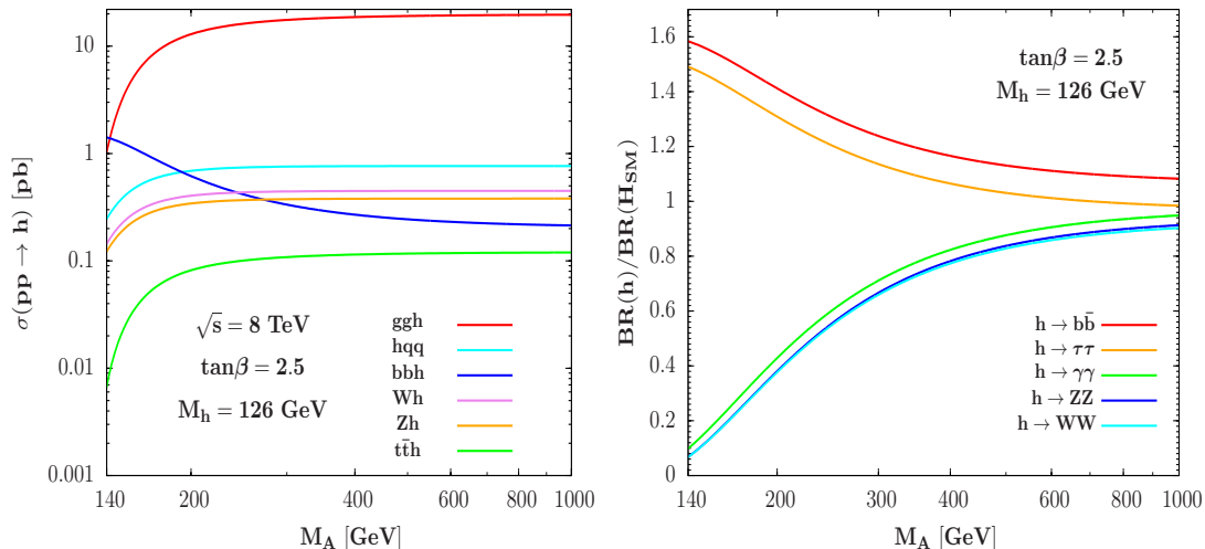
Figure 5. The production cross sections of the lighter h boson at the LHC with \sqrt{s} = 8 TeV (left) and the variation of its decay branching fractions compared to the SM values (right) for \tan\beta = 2.5 . Again, the radiative corrections in the Higgs sector are such that M_h = 126 GeV.
