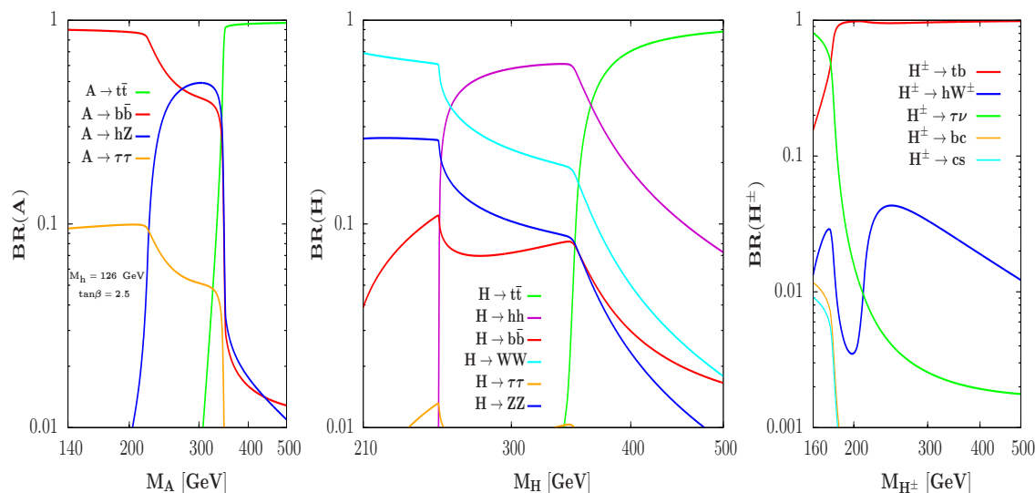
Figure 4. The decay branching ratios of the heavier MSSM Higgs bosons A (left), H (center) and H^\pm (right) as a function of their masses for \tan\beta = 2.5 . The program HDECAY [120, 121] has been used with modifications so that the radiative corrections lead to M_h = 126 GeV.
