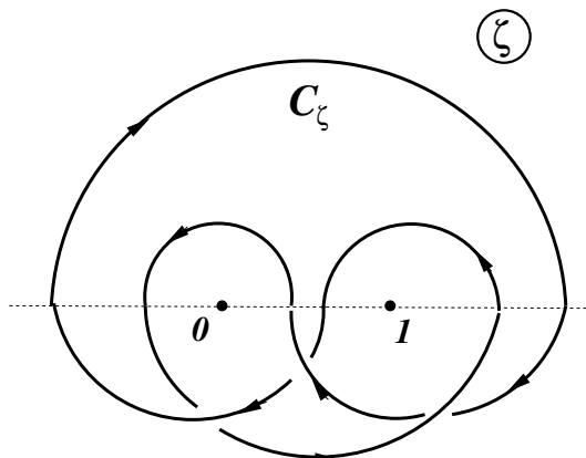
Figure 5. The Pochhammer loop C_\zeta appearing in (A.24).
