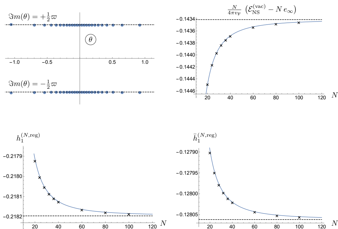
Figure 2. Numerical data for the ground state of the Hamiltonian \mathbb{H} (12.19) for even N/2 and S^z = 0 . The top left panel depicts the pattern of Bethe roots in the complex \theta plane with \theta = -\frac{1}{2} \log(\zeta) ( N = 100 ). The top right panel concerns the ground state energy \mathcal{E}_{\text{NS}}^{(\text{vac})} . The black crosses were obtained through the solution of the Bethe ansatz equations for increasing N , while the blue solid line represents the fit -0.14341 - 0.43286/N^2 . The limiting value, as predicted by eq. (12.45), is marked by the dashed black line. The bottom two panels illustrate the sum rules (12.38) and (12.40). The superscript “reg” indicates that a subtraction and rescaling has been made, which makes the limit N \rightarrow \infty well defined, e.g., h_1^{(N,\text{reg})} = N^{-(1-\beta^2)} \left( h_1^{(N)} - \frac{N}{2} \frac{\cos(\varpi)}{\sin(\pi\beta^2/2)} \right) . Again, the crosses stand for the numerical values, which were found by solving the Bethe ansatz equations, while the solid blue line is a fit, -0.21820 + 0.11285/N^2 and -0.12806 + 0.06623/N^2 for the bottom left and bottom right panels, respectively. The dashed line represents the limiting value according to eqs. (12.38) and (12.40). For the eigenvalue of the first non-local IM on the primary states, see (9.61) and (9.62). The parameters were taken to be \beta^2 = 0.43 , k = 0.1 and \varpi = 1.3 .
