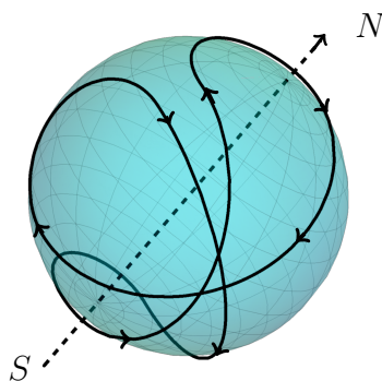
Figure 1. The Pochhammer loop on the Riemann sphere.
