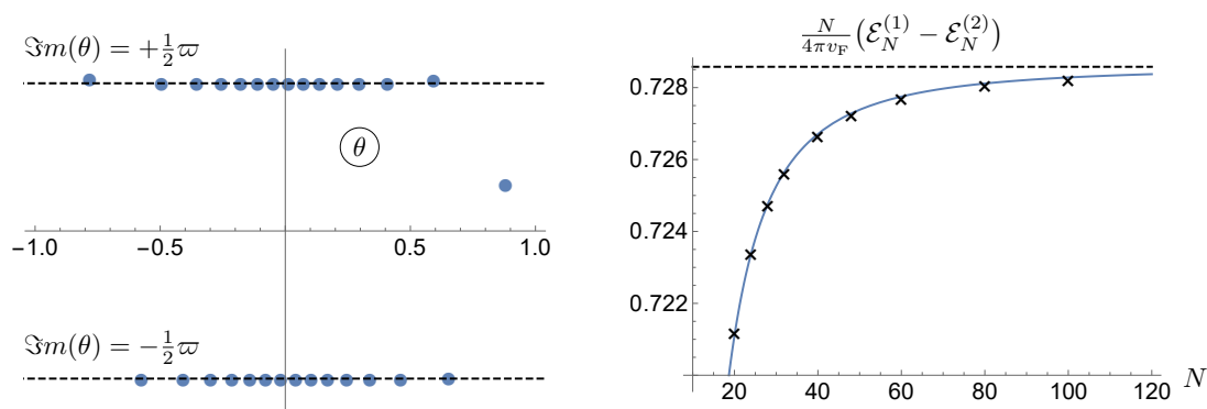
Figure 4. The first excited states of the Hamiltonian \mathbb{H} with N/2 even and S^z = 0 form a doublet. The Bethe roots for the states in the doublet are related to each other via complex conjugation. Depicted in the left panel of the figure is the typical pattern of Bethe roots in the complex \theta plane for the Bethe state, which flows to \bar{\mathbf{e}}_{1,+1}(\bar{P}_R^{(\text{vac})}) \otimes \mathbf{e}_{1,+1}(P_R^{(\text{vac})}) . The right panel compares the numerical data for the difference \mathcal{E}_N^{(1)} - \mathcal{E}_N^{(2)} with the prediction (12.61). The crosses were computed via the Bethe ansatz, while the solid blue line is the fit 0.72858 - 2.9919/N^2 . The dashed black line represents the r.h.s. of eq. (12.61). Note that, in the case at hand, I_1^{(e)} - \bar{I}_1^{(e)} is zero, while the eigenvalue of I_1^{(o)} on the Ramond primary states follows from eq. (9.19) and the last column of table 1. The parameters were set to be \beta^2 = 0.43 , \mathbf{k} = 0.1 and \varpi = 1.8 , so that P_R^{(\text{vac})} = -\bar{P}_R^{(\text{vac})} = -0.43133 .
