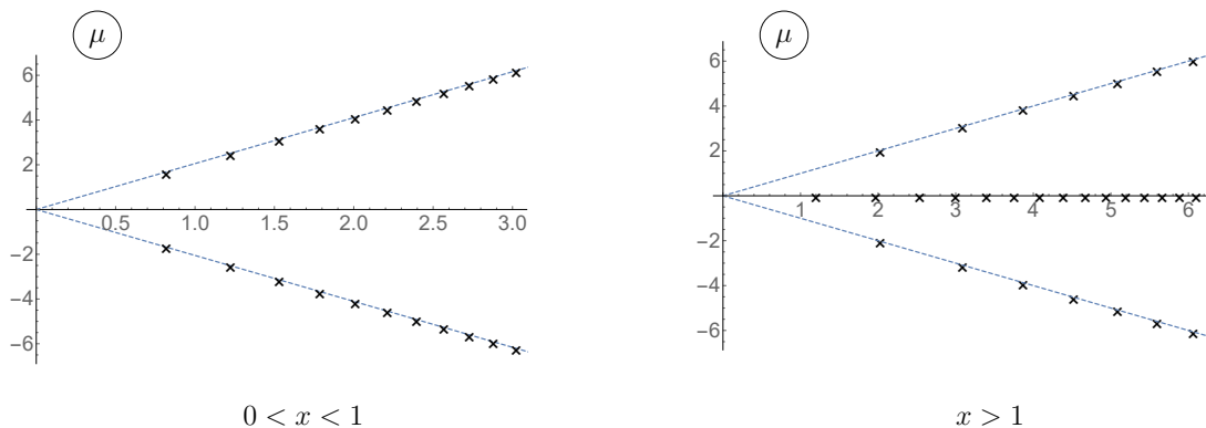
Figure 6. The typical pattern of zeroes of D_{j,m,A}(\mu) in the complex \mu plane for the two cases 0 < x < 1 and x > 1 . The numerical data was obtained for j_1 = j_2 = m = 0 , A = \frac{i}{2} and \xi = 1 , when the connection coefficient is expressed in terms of the parabolic cylinder function. The dashed lines mark the rays (B.4) and (B.13) in the left and right panels, respectively.
