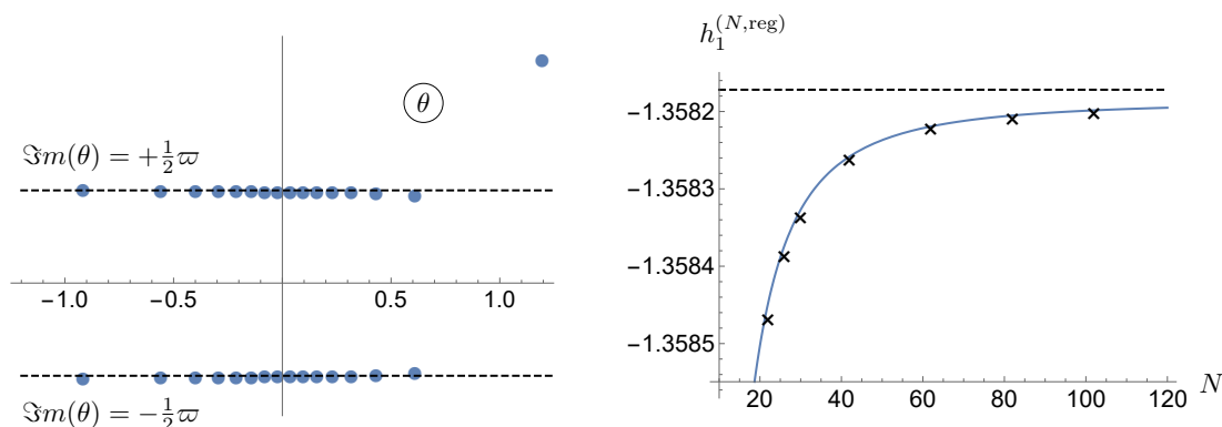
Figure 3. The left panel shows the typical pattern of Bethe roots in the complex \theta plane ( \theta = -\frac{1}{2} \log(\zeta) ) for the ground state of \mathbb{H} with N/2 odd and S^z = 0 , which flows to \bar{\mathbf{e}}_{0,0}(\bar{P}_{\text{NS}}^{(\text{vac})}) \otimes \mathbf{e}_{2,0}^{(-)}(P_{\text{NS}}^{(\text{vac})}) . Note that the right most root, located far above the real axis, has \Im m(\theta) = \frac{\varpi}{2} . The right panel presents numerical data for h_1^{(N,\text{reg})} = N^{-(1-\beta^2)} (h_1^{(N)} - \frac{N}{2} \frac{\cos(\varpi)}{\sin(\pi\beta^2/2)}) . The crosses were obtained from the solution of the Bethe ansatz equations, while the solid blue line represents the fit -1.3582 - 0.12659/N^2 . Formula (12.38) relates the limiting value \lim_{N \rightarrow \infty} h_1^{(N,\text{reg})} to the eigenvalue of the first non-local IM corresponding to the state \mathbf{e}_{2,0}^{(-)}(P_{\text{NS}}^{(\text{vac})}) . This eigenvalue is not available in analytical form. A numerical integration of the ODE (7.7) corresponding to \mathbf{e}_{2,0}^{(-)} leads to the prediction h_1^{(\infty)} = -1.35817 , which is depicted by the black dashed line. The parameters were set to be \beta^2 = 0.43 , \mathbf{k} = 0.1 and \varpi = 1.3 .
