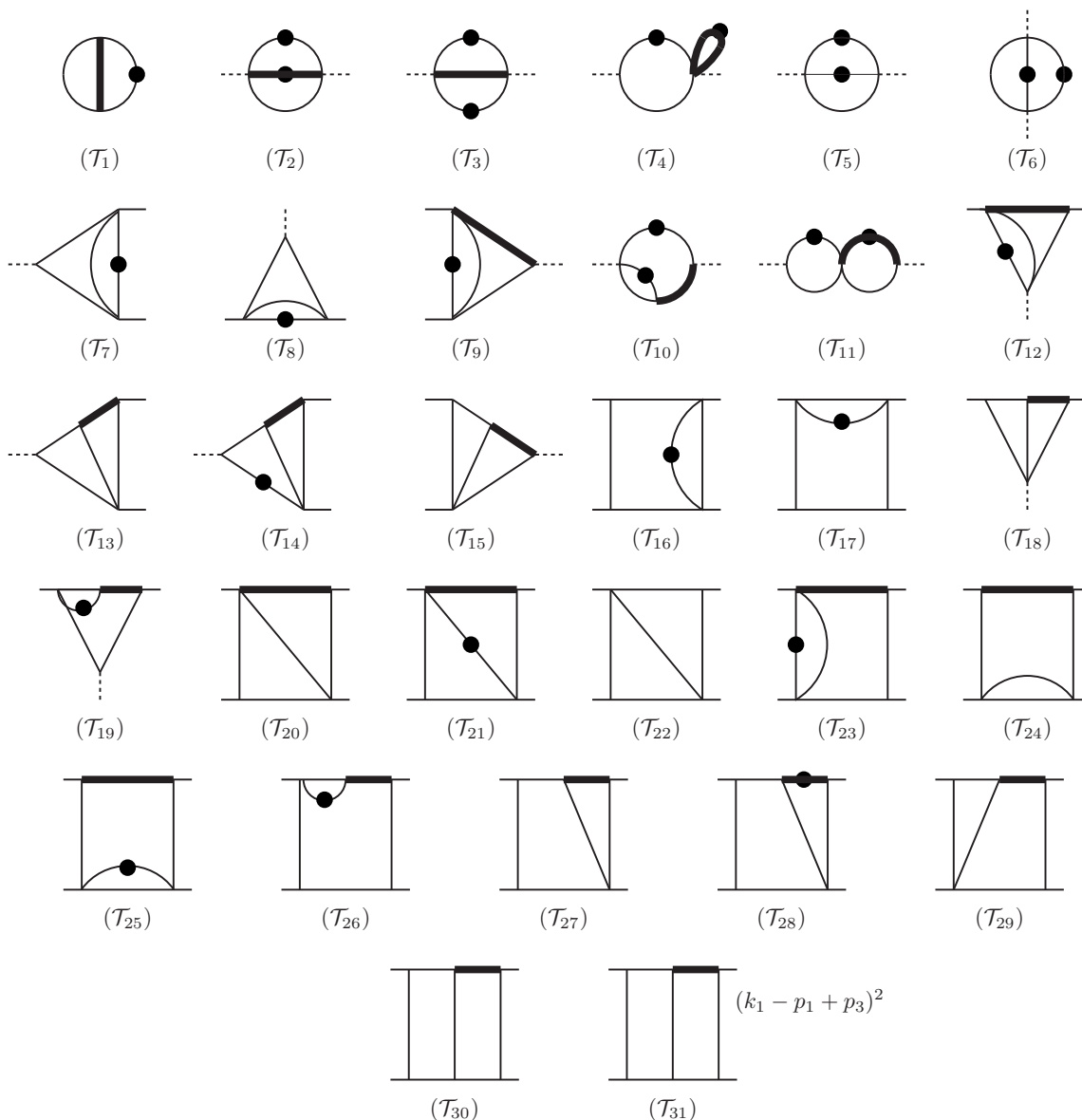
Figure 4. Two-loop one-mass MIs \mathcal{T}_{1,\dots,31} . The conventions are as in figure 3.
