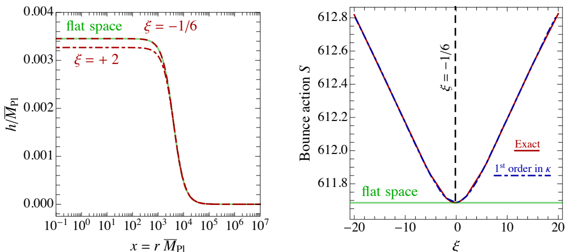
Figure 2. SM bounce solutions for different values of \xi (left panel), and their action (right panel). We consider M_h = 114 GeV, which is the value that saturates the meta-stability bound for the central value of the top mass. The bounce is sub-Planckian, so that gravitational corrections can be computed perturbatively.
