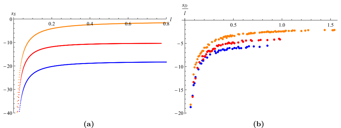
Figure 7. (a) The finite part of the entanglement entropy s_S as a function of the strip width l for the PMD with B/\phi_1^2 = 0.4183 (blue/lower), B/\phi_1^2 = 0.6710 (red/middle), and B/\phi_1^2 = 1.6383 (orange/upper). (b) The finite part of s_D/l as a function of l for the same value of the UV parameters with the same colors/locations. See footnote 6 for an explanation of the numerical variance in (b).
