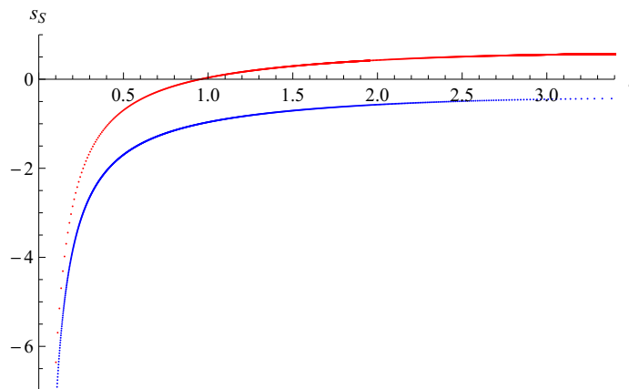
Figure 3. The finite part of the entanglement entropy s_S as a function of the strip width \ell for the numerical PED (blue/lower), with \delta f = 0 , and the analytical solution (red/upper), eqs. (4.4). We have taken our UV cutoff to be \epsilon = 10^{-5} and our maximal IR value of z_T = 0.9999 . See text for explanation of the shift.
