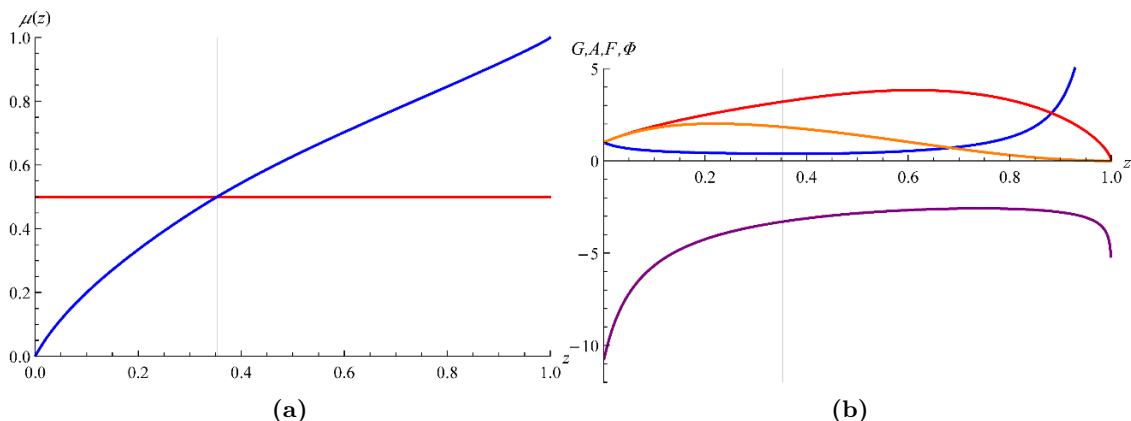
Figure 13. (a) The local chemical potential is shown in blue (the curve), where the fermion mass (shown in red, a horizontal line) is \tilde{m} = 0.5 and z_{star} = 0.3529 is the vertical line. The dual UV field theory parameters are B/\mu^2 = 6.8132 , Q/\mu^2 = 0.1136 , \phi_1/\mu = -3.6507 , and \phi_2/\mu^2 = 12.4852 . (b) The background metric and dilaton (lowest purple curve) for the same UV parameters as in (a). Here we have actually plotted G(z) = z^2g(z) , A(z) = z^2a(z) , and F(z) = z^2f(z) (lower-middle blue curve, upper red curve, and upper-middle orange curve respectively) so that our expect UV behavior is that each metric function goes to 1. We have also pulled out a factor of z in \Phi(z) , redefining \Phi(z) \rightarrow z\Phi(z) (purple). The vertical line is z_{star} .
