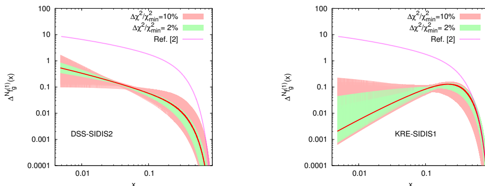
Figure 3. First k_{\perp} -moment of the gluon Sivens function as defined in eq. (2.11) for the SIDIS2 set (left panel) and SIDIS1 set (right panel) at Q^2 = 2 \text{ GeV}^2 . The best estimates (red solid lines) are shown together with the tolerance bands corresponding to a 2% (narrower, green) and 10% (wider, red) variation in the \chi^2 . The former bound on the gluon Sivens function (magenta dotted line), obtained in ref. [2], is also shown.
