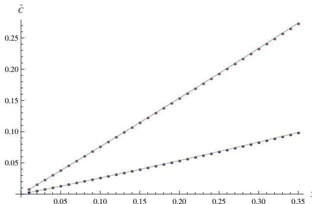
Figure 1. \tilde{C} = 1 - C_2(y)/C_2(0) as a function of y . There are two solutions (dots) approximated by eq. (3.32).
