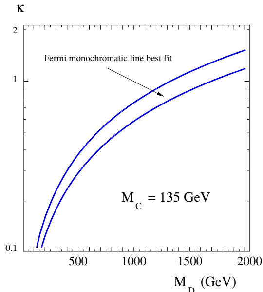
Figure 5. Parameter space (between the lines) satisfying \langle\sigma v\rangle_{\gamma\gamma} = (1.27 \pm 0.32_{-0.28}^{+0.18}) \times 10^{-27} \text{ cm}^3\text{s}^{-1} and fitting the tentative FERMI gamma-ray line at 135 GeV.
