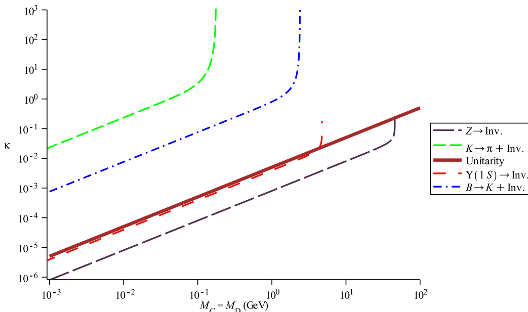
Figure 1. Bounds on \kappa . The unitarity bound assumes \Lambda = 1 TeV.
