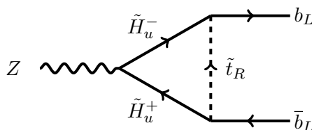
Figure 3. Loop diagram correcting R_b . The operators that are generated are W_{\mu\nu}^i Q_3^\dagger \sigma^i \bar{\sigma}^\mu i D^\nu Q_3 and B_{\mu\nu} Q_3^\dagger \bar{\sigma}^\mu i D^\nu Q_3 .
