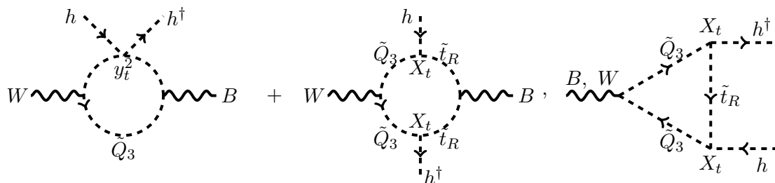
Figure 2. Loop diagrams contributing to the S parameter. The two diagrams at left generate the usual operator h^\dagger W^{i\mu\nu} \sigma^i h B_{\mu\nu} when the left-handed stop/sbottom doublet \tilde{Q}_3 and the right-handed stop \tilde{t}_R = (\tilde{u}_3^\dagger)^\dagger are integrated out. The diagram at right generates the operators i\partial^\nu B_{\mu\nu} h^\dagger \overleftrightarrow{D}^\mu h and iD^\nu W_{\mu\nu}^i h^\dagger \sigma^i \overleftrightarrow{D}^\mu h , which also contribute to S after being rewritten in terms of the minimal basis of dimension-six operators.
