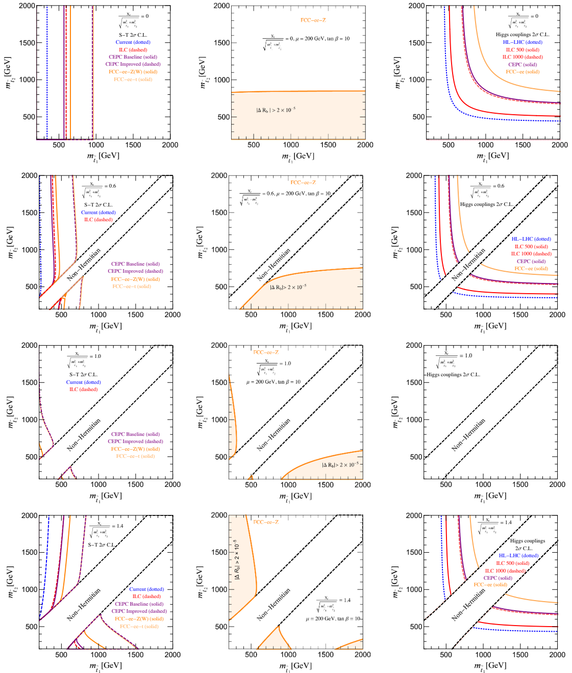
Figure 5. Regions in the stop physical mass plane that are/will be excluded at 2\sigma by EWPT with oblique corrections (left column), R_b at FCC-ee (mid column) and Higgs couplings (right column) for different choices of X_t/\sqrt{m_{\tilde{t}_1}^2 + m_{\tilde{t}_2}^2} : 0 (first row), 0.6 (2nd row), 1.0 (3rd row) and 1.4 (last row). We chose the mass eigenstate with m_{\tilde{t}_1} to be mostly left-handed while the mass eigenstate with m_{\tilde{t}_2} to be mostly right-handed. For non-zero choices of X_t , there are regions along the diagonal line which cannot be attained by diagonalizing a Hermitian mass matrix [32]. Also notice that the vacuum instability bound constrains X_t/\sqrt{m_{\tilde{t}_1}^2 + m_{\tilde{t}_2}^2} \lesssim \sqrt{3} [76].
