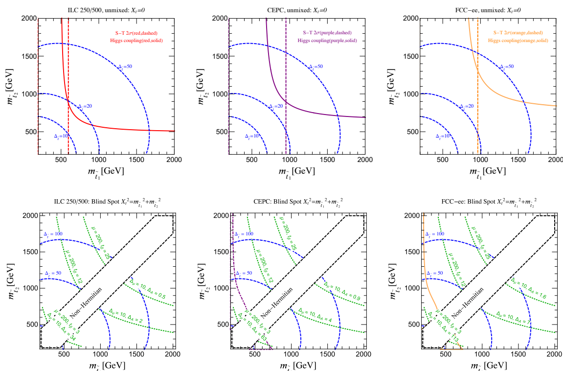
Figure 8. Regions in the physical stop mass plane that precision measurements are sensitive to, with contours of tunings, at future e^+e^- colliders (left: ILC; middle: CEPC; right: FCC-ee). Top row: bounds on stops with no mixing, X_t = 0 . Dashed vertical lines: 2\sigma bounds on stop masses from S and T (mostly T ); solid lines: 2\sigma bounds on stop masses from Higgs coupling constraints. Blue dashed contours are the stop contributions to the Higgs mass tuning. Lower row: bounds on stops in the blind spot X_t^2 = m_{t_1}^2 + m_{t_2}^2 . There are no Higgs measurement constraints. For CEPC with possible improvements (purple dash-dotted line in the middle) or FCC-ee (orange solid line), EWPT is only sensitive to a small region. The green dashed lines are the exclusion contours from b \rightarrow s\gamma for the choice \mu = 200 GeV and a few different values of \tan\beta . Each of these contours is also labeled with corresponding tunings \Delta_\mu and \Delta_A . There is also a region along the diagonal line which cannot be attained by diagonalizing a Hermitian mass matrix [32].
