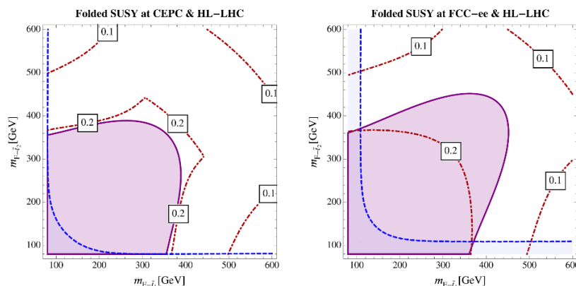
Figure 9. Projected constraints in the folded stop mass plane from a one-parameter fit to the Higgs-photon-photon couplings from future experiments. Directly analogous to figure 7. Results from the ILC 250/500/1000 would be similar to CEPC; lower-energy ILC measurements provide even weaker constraints. These constraints are subdominant to the constraints on left-handed folded stops arising from T -parameter measurements, which are the same as those for ordinary stops in the left-hand column of figure 5.
