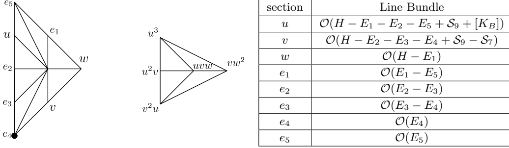
Figure 3. The toric diagram of polyhedron F_{13} and its dual. The zero section is indicated by the dot. In the accompanying table we indicate the divisor classes of the fiber coordinates.
