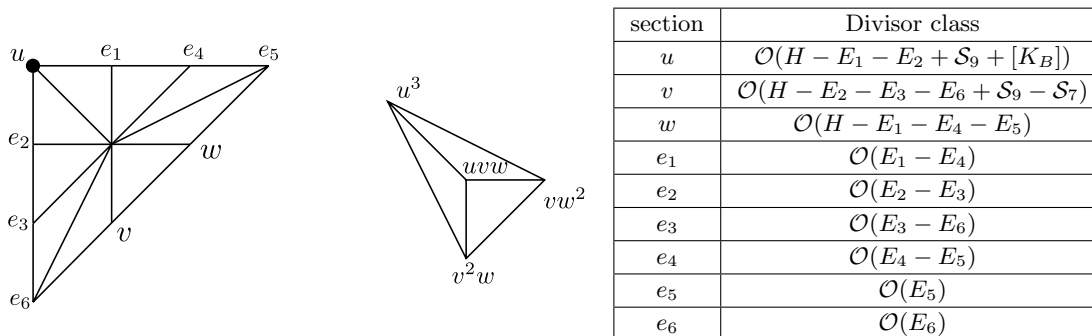
Figure 5. The toric diagram of polyhedron F_{16} and its dual. The zero section is indicated by the dot. In the accompanying table we indicate the divisor classes of the fiber coordinates.
