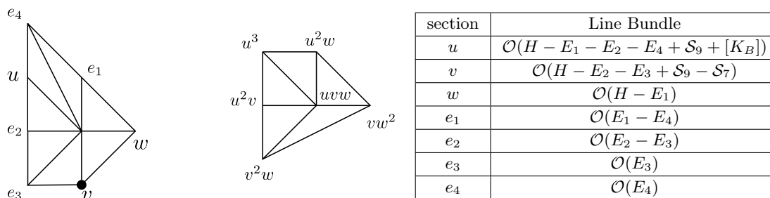
Figure 1. The toric diagram of polyhedron F_{11} and its dual. The zero section is indicated by the dot. In the accompanying table we indicate the divisor classes of the fiber coordinates.
