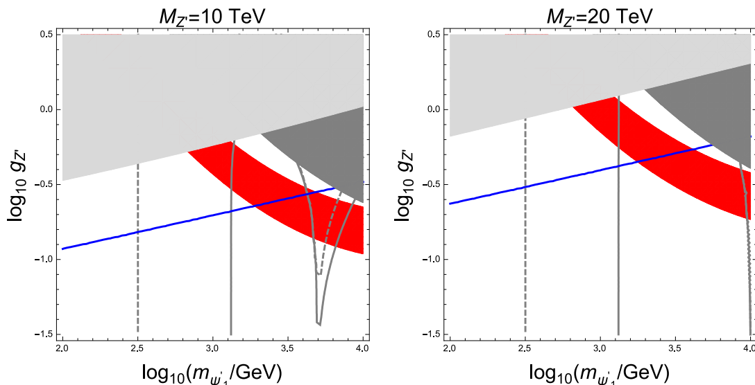
Figure 2. Plots in (m_{\psi'_1}, g_Z) -plane. The red-colored region can explain the 3.5 keV X-ray line signal. The dark gray region is excluded because the lifetime of \psi'_2 is shorter than the age of the universe. The light gray region is excluded by LUX DM direct detection experiment. The blue line is the sensitivity the next XENON1T experiment can reach. The black solid (dashed) line gives the correct relic abundance of DM for y_i = 2(1) . For the left (right) plot we set M_{Z'} = 10(20) TeV.
