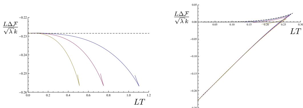
Figure 4. On the left is the plot of the free energy difference \frac{L\Delta\mathcal{F}}{\sqrt{\lambda}\kappa} as a function of LT obtained numerically. The dashed black line is the result obtained for an extremal probe ( \kappa = 0 ). On the right there is a plot for the same values of \kappa in the deconfined phase.
