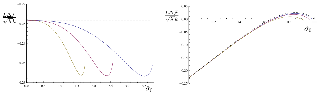
Figure 3. On the left is the plot of the free energy difference \frac{L\Delta\mathcal{F}}{\sqrt{\lambda}\kappa} as a function of \hat{\sigma}_0 obtained numerically. The dashed black line is the result obtained for an extremal probe ( \kappa = 0 ). On the right there is a plot for the same values of \kappa in the deconfined phase. The colour coding is the same as for the distances LT presented in the previous figures.
