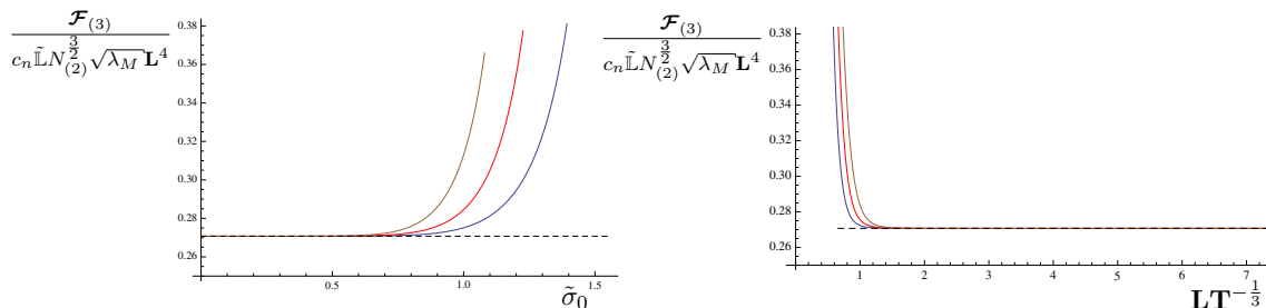
Figure 17. On the left we have plotted the free energy \mathcal{F}_{(3)} a function of \tilde{\sigma}_0 and on the right as a function of the distance L T^{-\frac{1}{3}} . The colour coding is the same as in the previous figure.
