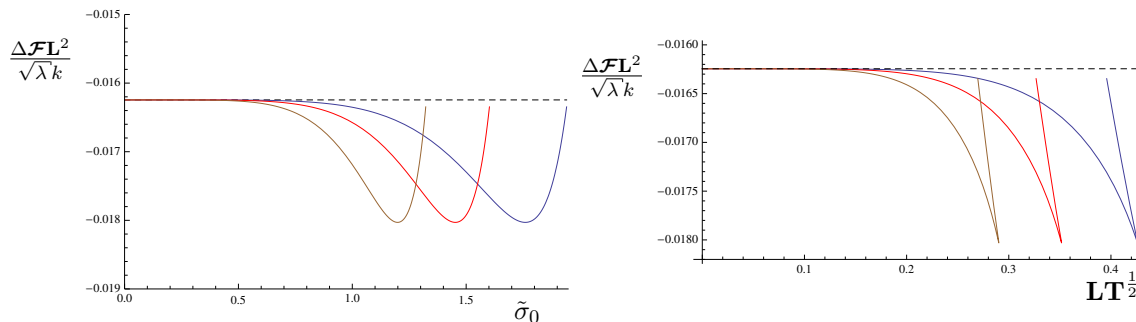
Figure 8. On the left is the plot of \frac{\Delta\mathcal{F}L^2}{\sqrt{\lambda}k} , where \Delta\mathcal{F} \equiv \mathcal{F}_{\text{loop}} - \mathcal{F}_{\text{W}\ell} , as function of \tilde{\sigma}_0 and as a function of \mathbf{L}T^{\frac{1}{2}} on the right. The colour coding is the same as on the l.h.s. of the previous figure. The dashed line is the result for \kappa = 0 .
