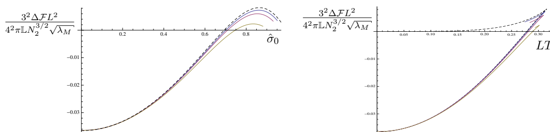
Figure 13. On the left we have the free energy difference as a function of \hat{\sigma}_0 and on the right as a function of LT in the case \gamma = 1 . The dashed line represents \bar{\kappa} = 0 and has been obtained in [32].
