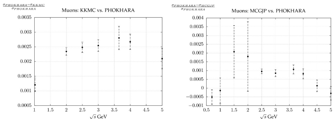
Figure 4. The size of the relative difference between PHOKHARA 8.0, KKMC 4.13 and MCGPJ for muon pair production.
