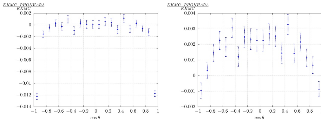
Figure 9. The relative difference of the angular distributions given by PHOKHARA 8.0 and KKMC 4.13. In the left plot no cuts are applied. In the right plot the events with the muon pair invariant mass Q^2 > 0.3 \text{ GeV} are selected.
