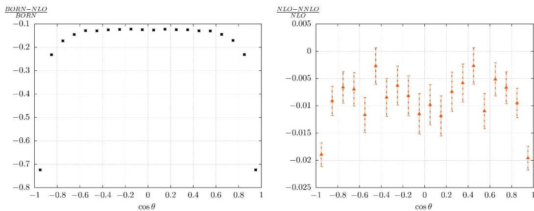
Figure 6. The size of NLO and NNLO corrections to the muon polar angle distribution.
