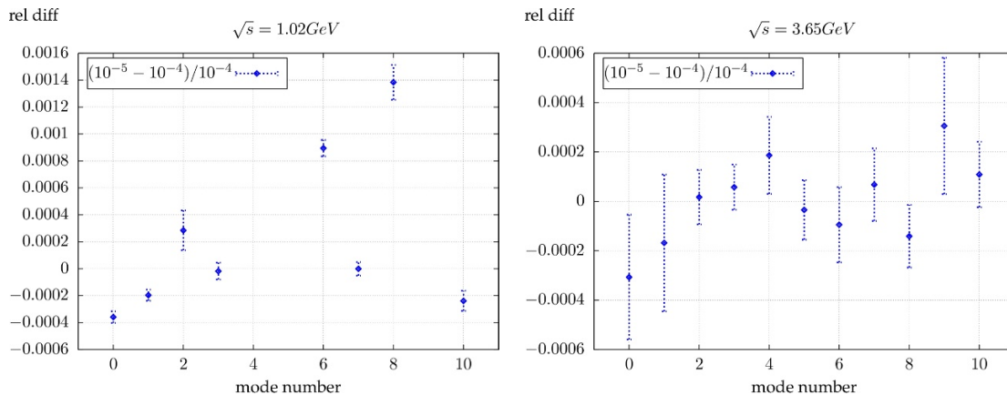
Figure 2. The difference between integrated cross sections with separation parameter w = 10^{-4} and w = 10^{-5} for 10 modes in PHOKHARA 8.0: 0 ( \mu^+\mu^- ), 1 ( \pi^+\pi^- ), 2 ( 2\pi^0\pi^+\pi^- ), 3 ( 2\pi^+2\pi^- ), 4 ( p\bar{p} ), 5 ( n\bar{n} ), 6 ( K^+K^- ), 7 ( K^0\bar{K}^0 ), 8 ( \pi^0\pi^+\pi^- ), 9 ( \Lambda(\rightarrow\pi^-p)\bar{\Lambda}(\rightarrow\pi^+\bar{p}) ), 10 ( \eta\pi^+\pi^- ).
