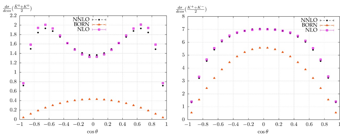
Figure 7. The size of NLO and NNLO corrections to the kaon polar angle distribution (left plot neutral kaons, right plot charged kaons).
