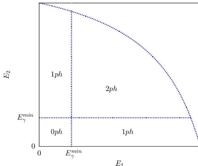
Figure 1. Division of contributions from two photon phase space into three parts of the cross section. 0ph -part is added into d\sigma(e^+e^- \rightarrow \text{hadrons}) ; 1ph -part is added into d\sigma(e^+e^- \rightarrow \text{hadrons} + \text{one hard photon}) ; 2ph -part is calculated in d\sigma(e^+e^- \rightarrow \text{hadrons} + \text{two hard photons}) .
