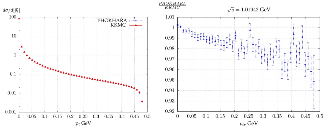
Figure 8. Comparison of the missing momentum distribution between PHOKHARA 8.0 and KKMC 4.13 for \sqrt{s} = 1.01942 GeV, which are indistinguishable in the left plot.
