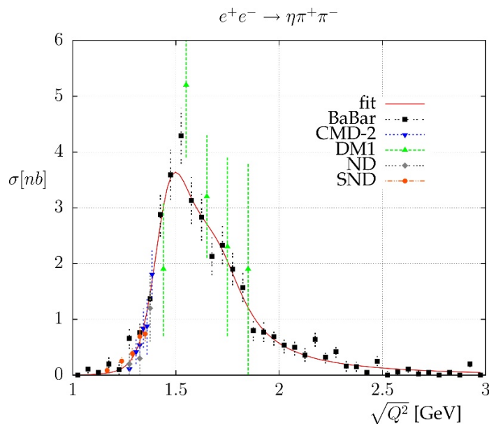
Figure 10. Fitted cross section of e^+e^- \rightarrow \eta\pi^+\pi^- and all experimental data used in the fit procedure: [41–45].
