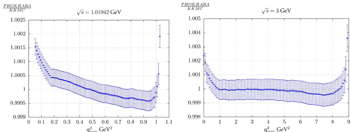
Figure 3. Ratio of the integrated cross section obtained by KKMC 4.13 and PHOKHARA 8.0 as a function of the lower limit of the muon pair invariant mass q_{\min}^2 .
