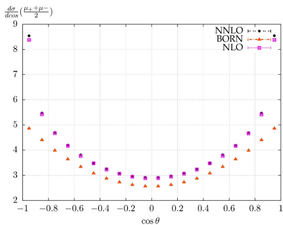
Figure 5. The size of NLO and NNLO corrections to the muon polar angle distribution.
