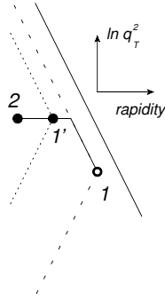
Figure 24. An emission limits the ordered phase space of the parents.
