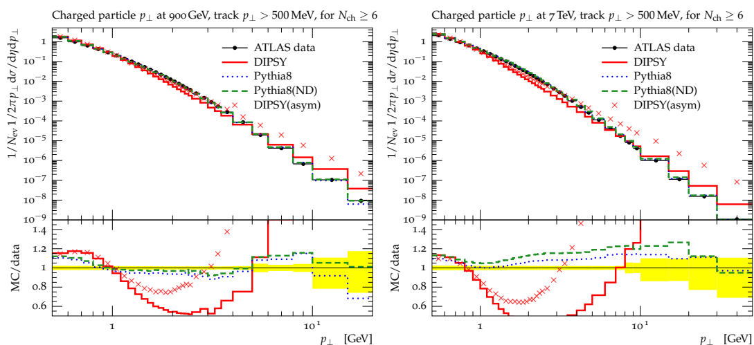
Figure 16. The transverse momentum distribution of charged particles at 0.9 (left) and 7 TeV (right). Data points and lines as in figure 15.
