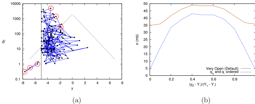
Figure 11. (a) Two colliding virtual cascades in the y - q_{\perp} representation, generated by the Monte Carlo in an off-central frame. The lines shows the colour flow between the partons, the dashed vertical line is the collision frame y_0 and the circled partons are the starting valence partons. The outside triangle show the incoming p_+ and p_- of the protons. (b) The frame dependence of the total pp cross section at \sqrt{s} = 200 GeV. The dashed curve has full q_{\pm} ordering in the interaction, the full one only requires enough energy to set the interaction on shell.
