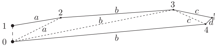
Figure 9. A cascade where the dipole sizes increase to a maximum, and then decrease. Here the size of the largest dipole, denoted b , corresponds to the minimum k_{\perp} in the chain.
