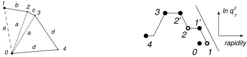
Figure 10. A cascade with a maximum in q_{\perp} where the small dipole corresponding to the large q_{\perp} , does not split. The outer q_{\perp} maximum is shown in impact-parameter space (left) and y - q_{\perp} space (right).
