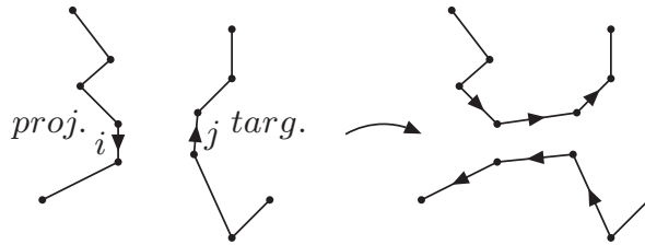
Figure 3. A dipole-dipole interaction implies exchange of colour and reconnection of the dipole chains in the colliding cascades. The arrows indicate the direction of the dipole going from colour charge to anticharge.
