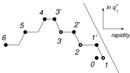
Figure 8. The same cascade as in figure 8. The x direction shows rapidity, and y direction shows \ln(k_\perp^2) . The diagonal line is the constant p_+ of the incoming particle.
