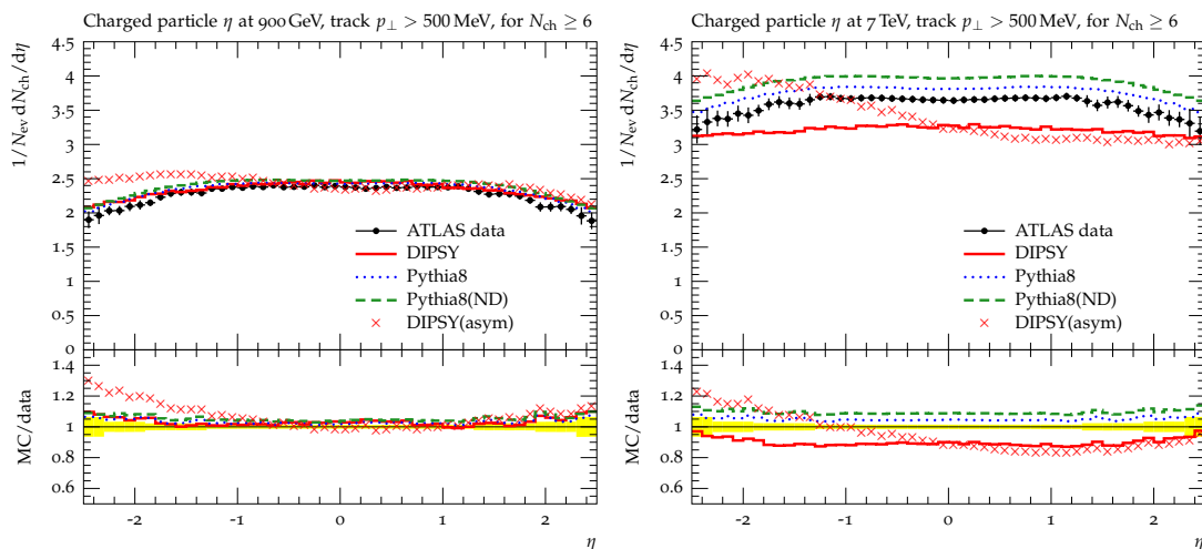
Figure 17. The pseudo-rapidity distribution of charged particles at 0.9 (left) and 7 TeV (right). Data points and lines as in figure 15.
