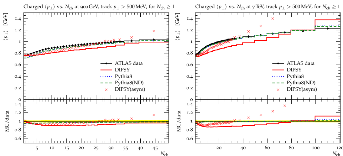
Figure 18. The average transverse momentum as a function of charged particle multiplicity at 0.9 (left) and 7 TeV (right). Data points and lines as in figure 15.
