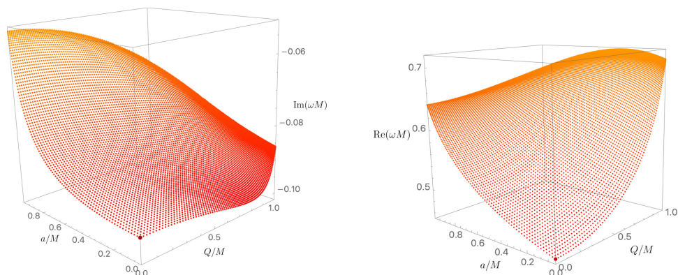
Figure 25. Imaginary (left panel) and real (right panel) parts of the frequency for the Z_1 , (\ell, m, n) = (2, 1, 0) KN PS QNM. The dark-red point ( a = 0 = Q ), \tilde{\omega} \simeq 0.45759551 - 0.09500443 i , is the gravitational QNM of Schwarzschild [40, 41].
