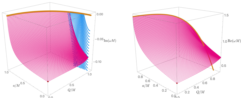
Figure 18. Imaginary (left panel) and real (right panel) parts of the frequency for the Z_2 , (\ell, m, n) = (3, 3, 0) KN PS QNM. The dark-red point ( a = 0 = Q ), \tilde{\omega} \simeq 0.59944329 - 0.09270305 i , is the gravitational QNM of Schwarzschild [40, 41]. The magenta surface describes PS_0 modes while the blue surface corresponds to the NH_0 modes.
