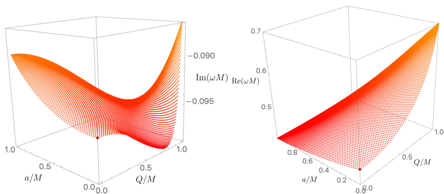
Figure 27. Imaginary (left panel) and real (right panel) parts of the frequency for the Z_1 , (\ell, m, n) = (2, -1, 0) KN PS QNM. The dark-red point ( a = 0 = Q ), \tilde{\omega} \simeq 0.45759551 - 0.09500443 i , is the gravitational QNM of Schwarzschild [40, 41].
