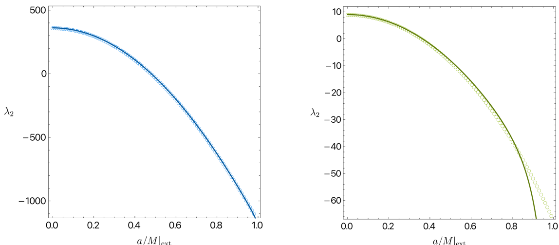
Figure 8. Comparing the WKB result (continuous line) for \lambda_2(m, \hat{a}) with the exact result (circles). Left panel: m = 10 case. Right panel: m = 2 case.
