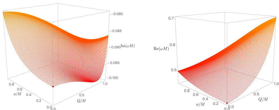
Figure 26. Imaginary (left panel) and real (right panel) parts of the frequency for the Z_1 , (\ell, m, n) = (2, 0, 0) KN PS QNM. The dark-red point ( a = 0 = Q ), \tilde{\omega} \simeq 0.45759551 - 0.09500443 i , is the gravitational QNM of Schwarzschild [40, 41].
