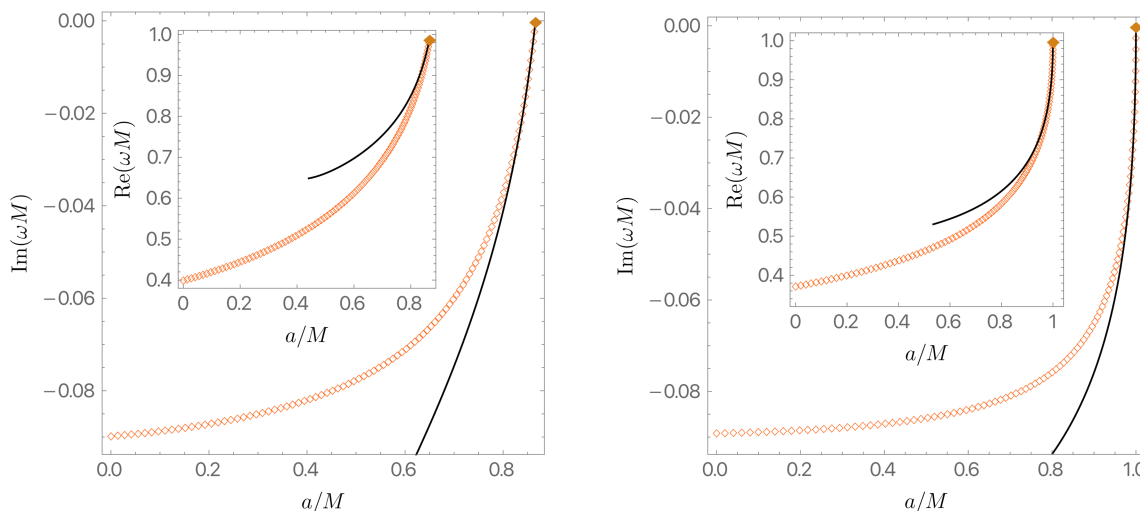
Figure 10. Imaginary and real (inset plot) part of the frequency as a function of the rotation for the PS QNM family with Q/r_+ = 0.5 (left panel) and Q = 0 (right panel). The numerical results are given by the orange diamonds while the black line is the analytical result (3.40). The brown diamond is the value \tilde{\omega} = m\tilde{\Omega}_H^{\text{ext}} at extremality. \tilde{\omega}_{\text{MAE}} in (3.40) is a good analytical approximation for those PS modes that approach \text{Im}\tilde{\omega} = 0 at extremality. The approximation (3.40) to the PS modes improves as \tilde{Q} decreases.
