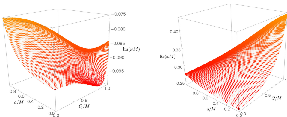
Figure 30. Imaginary (left panel) and real (right panel) parts of the frequency for the Z_1 , (\ell, m, n) = (1, 0, 0) KN PS QNM. The dark-red point ( a = 0 = Q ), \tilde{\omega} \simeq 0.24826326 - 0.09248772 i , is the gravitational QNM of Schwarzschild [40, 41].
