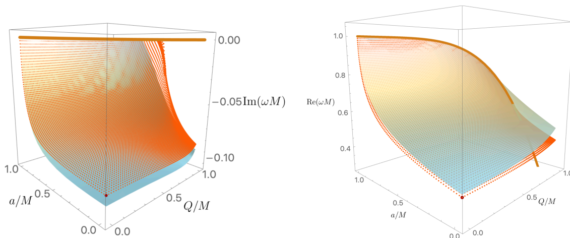
Figure 4. Comparing the eikonal prediction \omega_{\text{PS}}^{\text{eikn}} (light blue surface) with the actual numerical frequencies (orange points) for co-rotating PS modes with m = \ell = 2, n = 0 . The former is given by (3.11)–(3.16) with r_s = r_s^- of figure 2 and b_s > 0 . The brown curve at extremality has \text{Im} \tilde{\omega} = 0 and \text{Re} \tilde{\omega} = m \tilde{\Omega}_H^{\text{ext}} . Although m = 2 is certainly outside the regime of validity of the geometrics optics approximation, |m| \gg 1 , it turns out that the approximation (3.16) proves to be reasonably good. The dark-red point at (\tilde{Q}, \tilde{a}) = (0, 0) coincides with the Schwarzschild QNM, \tilde{\omega} \simeq 0.37367168 - 0.08896232 i , first computed in [40, 41].
