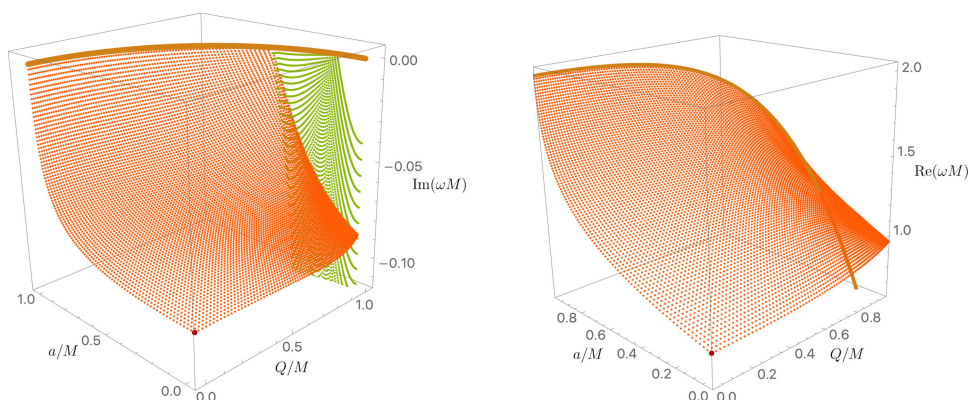
Figure 19. Imaginary (left panel) and real (right panel) parts of the frequency for the Z_2 , (\ell, m, n) = (4, 4, 0) KN PS QNM. The dark-red point ( a = 0 = Q ), \tilde{\omega} \simeq 0.80917838 - 0.09416396 i , is the gravitational QNM of Schwarzschild [40, 41]. The orange surface describes PS_0 modes while the green surface corresponds to the NH_0 modes.
