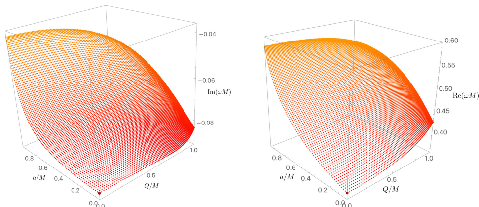
Figure 21. Imaginary (left panel) and real (right panel) parts of the frequency for the Z_2 , (\ell, m, n) = (2, 1, 0) KN PS QNM. The dark-red point ( a = 0 = Q ), \tilde{\omega} \simeq 0.37367168 - 0.08896232 i , is the gravitational QNM of Schwarzschild [40, 41].
