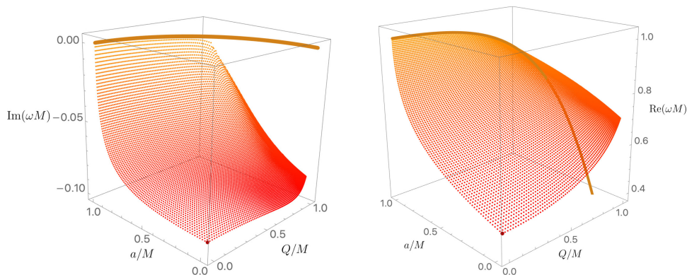
Figure 24. Imaginary (left panel) and real (right panel) parts of the frequency for the Z_1 , (\ell, m, n) = (2, 2, 0) KN PS QNM. The dark-red point ( a = 0 = Q ), \tilde{\omega} \simeq 0.45759551 - 0.09500443 i , is the gravitational QNM of Schwarzschild [40, 41].
