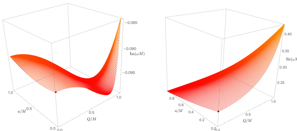
Figure 31. Imaginary (left panel) and real (right panel) parts of the frequency for the Z_1 , (\ell, m, n) = (1, -1, 0) KN PS QNM. The dark-red point ( a = 0 = Q ), \tilde{\omega} \simeq 0.24826326 - 0.09248772 i , is the gravitational QNM of Schwarzschild [40, 41].
