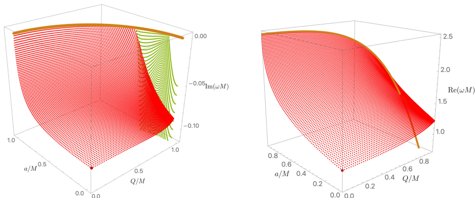
Figure 20. Imaginary (left panel) and real (right panel) parts of the frequency for the Z_2 , (\ell, m, n) = (5, 5, 0) KN PS QNM. The dark-red point ( a = 0 = Q ), \tilde{\omega} \simeq 1.01229531 - 0.09487052 i , is the gravitational QNM of Schwarzschild [40, 41]. The red surface describes PS_0 modes while the green surface corresponds to the NH_0 modes.
