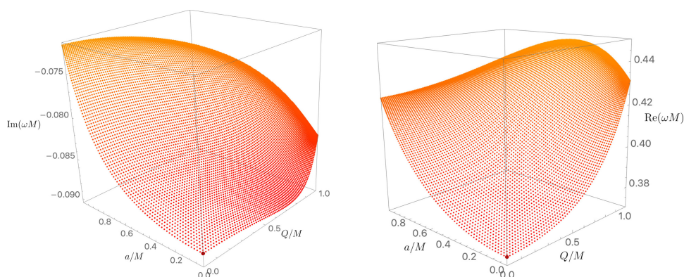
Figure 22. Imaginary (left panel) and real (right panel) parts of the frequency for the Z_2 , (\ell, m, n) = (2, 0, 0) KN PS QNM. The dark-red point ( a = 0 = Q ), \tilde{\omega} \simeq 0.37367168 - 0.08896232 i , is the gravitational QNM of Schwarzschild [40, 41].
