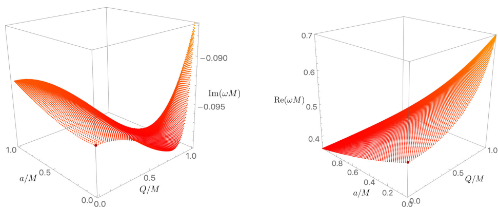
Figure 28. Imaginary (left panel) and real (right panel) parts of the frequency for the Z_1 , (\ell, m, n) = (2, -2, 0) KN PS QNM. The dark-red point ( a = 0 = Q ), \tilde{\omega} \simeq 0.45759551 - 0.09500443 i , is the gravitational QNM of Schwarzschild [40, 41].
