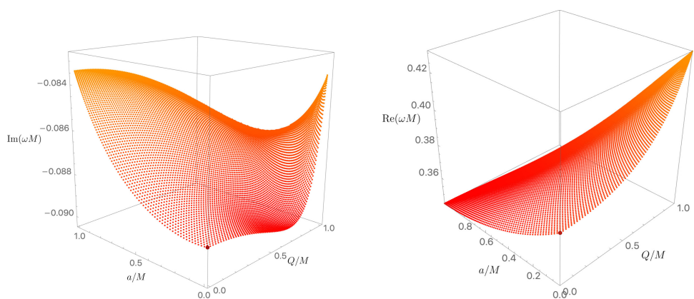
Figure 23. Imaginary (left panel) and real (right panel) parts of the frequency for the Z_2 , (\ell, m, n) = (2, -1, 0) KN PS QNM. The dark-red point ( a = 0 = Q ), \tilde{\omega} \simeq 0.37367168 - 0.08896232 i , is the gravitational QNM of Schwarzschild [40, 41].
