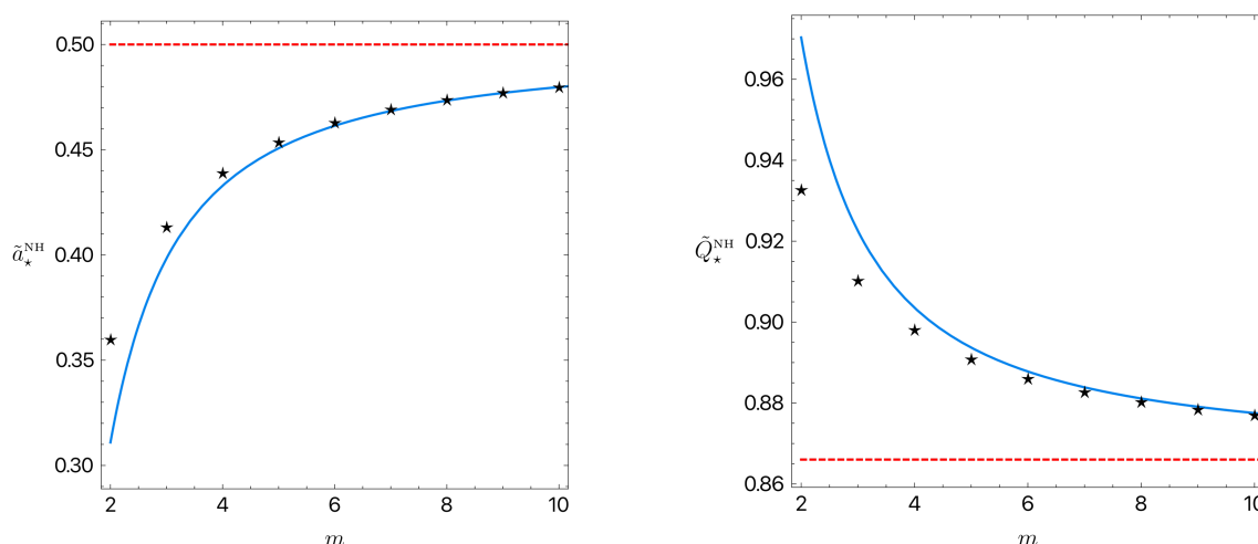
Figure 11. Critical values of \tilde{a}_\star^{\text{NH}} (left panel) and \tilde{Q}_\star^{\text{NH}} (right panel) for which \lambda_2 vanishes as a function of m . The WKB approximation (3.41) (blue line) already gives an excellent agreement with the exact results (black \star 's) for values of m as low as 5 or 6. Further note that as m increases, \tilde{a}_\star^{\text{NH}} \rightarrow \tilde{a}_\star^{\text{eikn}} = \frac{1}{2} (left panel) and \tilde{Q}_\star^{\text{NH}} \rightarrow \tilde{Q}_\star^{\text{eikn}} = \frac{\sqrt{3}}{2} (right panel) — see the red dashed lines — where the latter eikonal values were discussed in figure 5 (see its red \star point).
