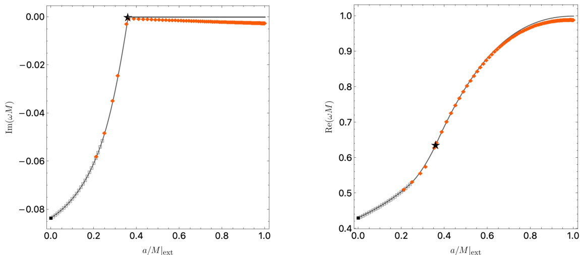
Figure 12. The PS modes at extremality. The black \star at \tilde{a}_{\text{ext}} = \tilde{a}_\star \simeq 0.360 is the one shown in figure 11. The grey squares in the range \tilde{a}_{\text{ext}} \in [0, 0.24] describe data obtained solving the gravito-electromagnetic PDEs directly at extremality . The grey line in the range \tilde{a}_{\text{ext}} \in [0, \tilde{a}_\star] is an interpolation of the grey square and \star points. On the other hand, for \tilde{a}_{\text{ext}} > \tilde{a}_\star it is simply described by \text{Im} \tilde{\omega} = 0 and \text{Re} \tilde{\omega} = m \tilde{\Omega}_H^{\text{ext}} . The orange diamonds describe the closest point to extremality we obtained using the non-extremal code. Left panel: imaginary part of the PS frequency. Right panel: real part of the PS frequency.
