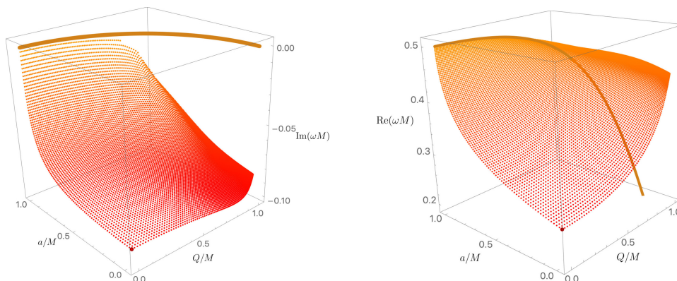
Figure 29. Imaginary (left panel) and real (right panel) parts of the frequency for the Z_1 , (\ell, m, n) = (1, 1, 0) KN PS QNM. The dark-red point ( a = 0 = Q ), \tilde{\omega} \simeq 0.24826326 - 0.09248772 i , is the gravitational QNM of Schwarzschild [40, 41].
