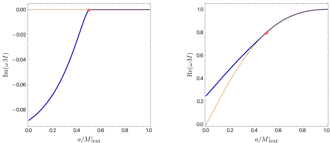
Figure 5. The eikonal prediction for (3.16) for \omega_{\text{PS}}^{\text{eikn}} evaluated at extremality (dark-blue line). The dotted brown line has \text{Im} \tilde{\omega} = 0 and \text{Re} \tilde{\omega} = m \tilde{\Omega}_H (they correspond to the solid brown lines in figures 3–4). The red \star point is at \tilde{a}_{\text{ext}} = \tilde{a}_\star^{\text{eikn}} = \frac{1}{2} .
