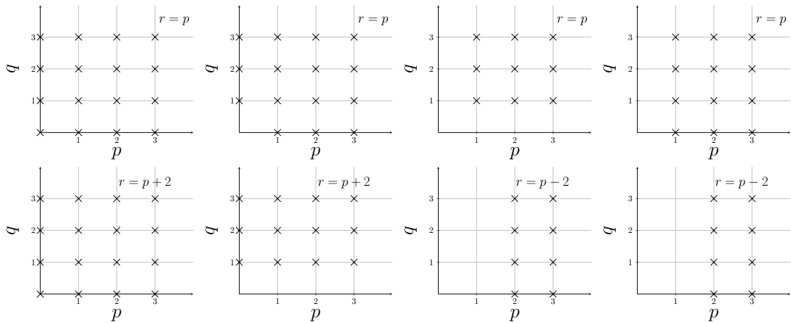
Figure 8. \mathcal{D}_{1/2} towers.
