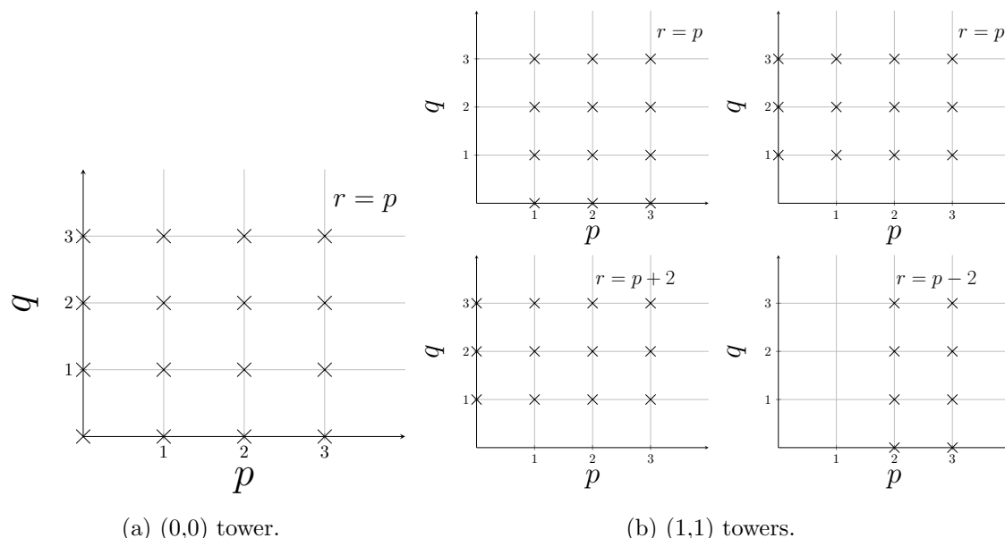
Figure 1. (0,0) and (1,1) towers.
