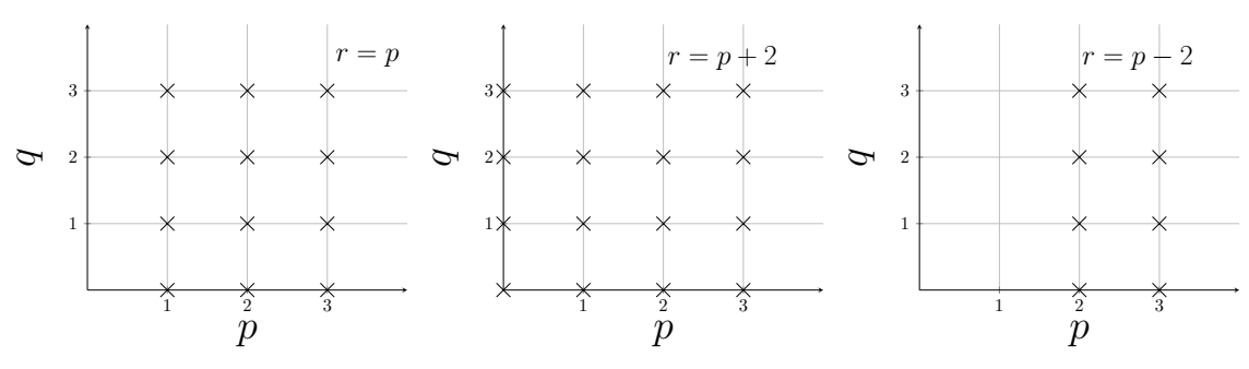
Figure 2. (0,2) towers.
