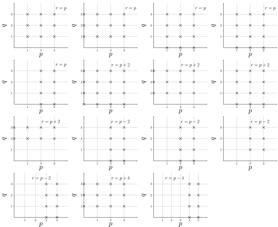
Figure 9. Two-form towers.
