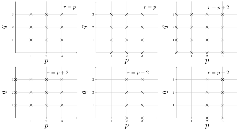
Figure 7. One-form towers.
