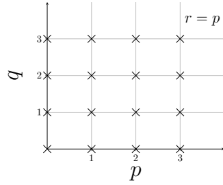
Figure 6. Scalar tower.
