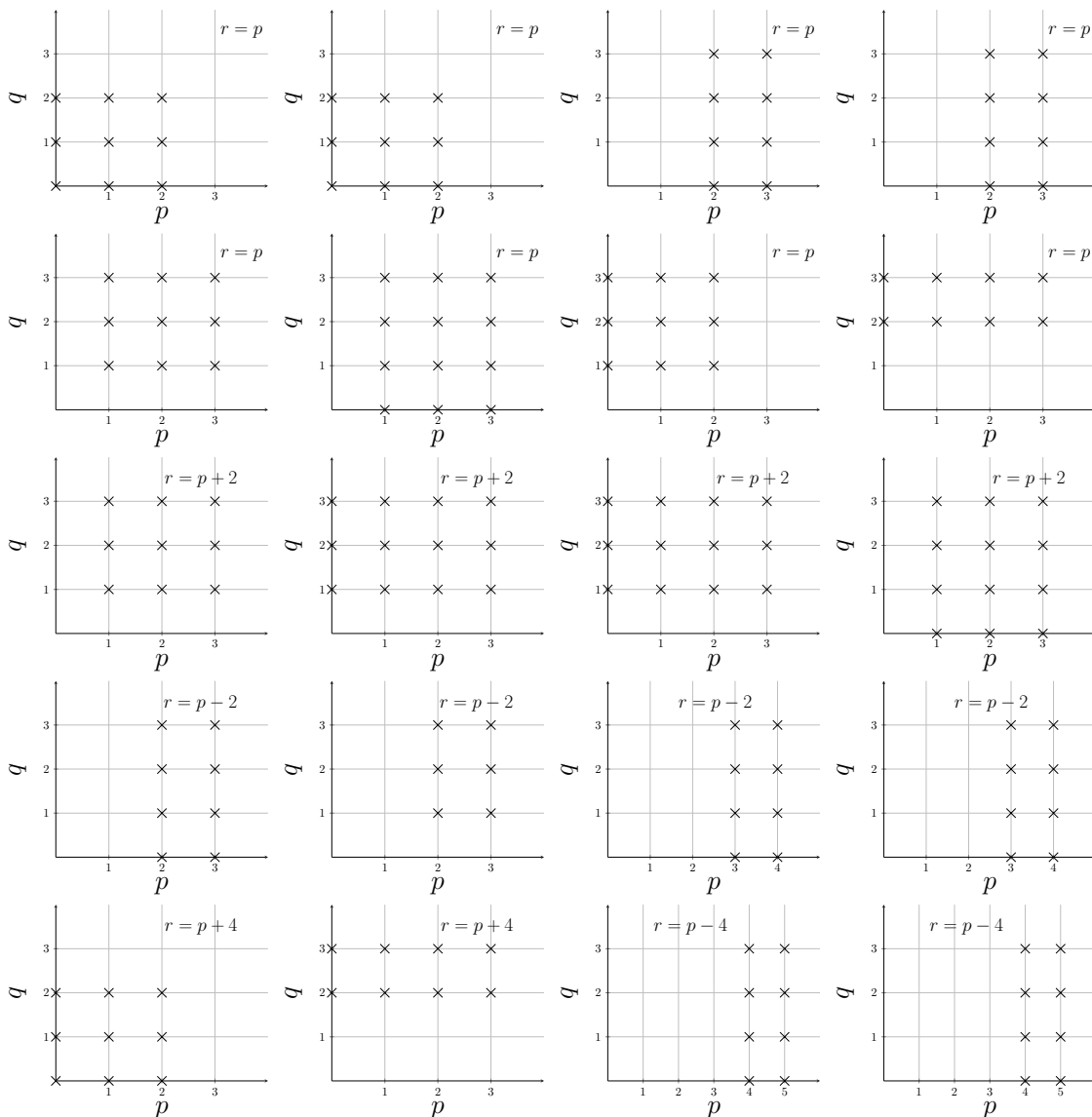
Figure 12. Q towers.
