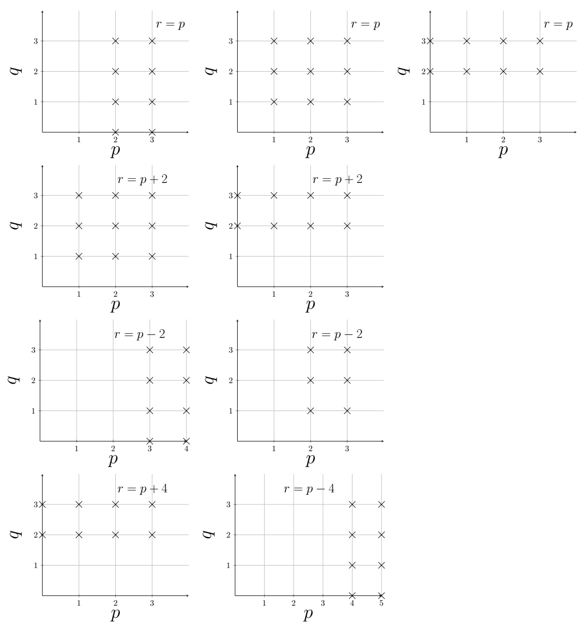
Figure 5. (2,2) towers.
