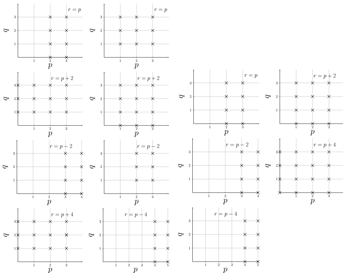
(a) (1,3) towers.
