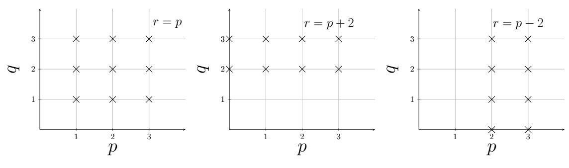
Figure 3. (2,0) towers.
