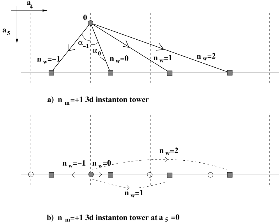
Figure 3. Monopole-instanton solutions for n_m = +1 are represented by a line with an arrow pointing from the vev of a_{4,5} at the center of the monopole, denoted by a circle, to the vev at infinity, denoted by a square (the vev at the center vanishes and is, on both pictures, taken to be the origin of coordinates in the a_4/a_5 -plane). Since a_4 is an angular variable on \mathbb{R}^3 \times \mathbb{S}^1 , a tower of instanton-monopoles of “winding numbers” labelled by n_w exists. The length of the arrow equals the distance between the vevs at the center of the monopole and infinity, \sqrt{a_5^2 + a_4(n_w)^2} , and is proportional to the action of the corresponding topological defect. The n_m = +1 tower, shown in the upper figure, is composed of deformations (obtained by turning on a_5 ) of BPS monopole-instantons and \overline{\text{KK}} twisted anti-instantons, shown in the lower figure (BPS monopoles have their arrows pointing to the right and \overline{\text{KK}} -monopoles to the left). The n_m = -1 tower, not shown above, obtained by reverting all the arrows, is composed of deformations of \overline{\text{BPS}} anti-monopole-instantons and \text{KK} twisted monopole-instantons.
