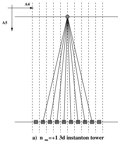
Figure 4. 3d-instantons in the magnetic charge +1 tower in the regime a_4 \ll a_5 \ll a_4/g_4^2 . The tower is composed of deformation of BPS monopole instantons and \overline{KK} twisted anti-instantons. The properties of fermionic zero modes is dictated by the leading a_5 dependence for the low winding number instantons.
