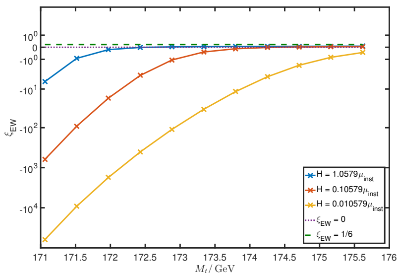
Figure 9. Plot of the boundary between stability and instability for different Hubble rates, and top masses. Note that \mu_{inst} is defined by \lambda(\mu_{inst}) = 0 using m_t = 173.34 \text{ GeV} for comparison. Note that since the results in this paper use only 1-loop running, low values of m_t can be unstable for values that would lead to an absolutely stable vacuum at 3-loops.
