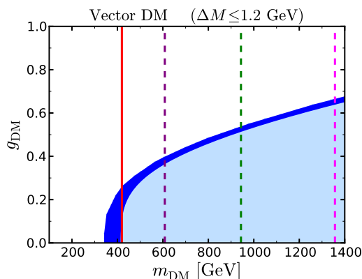
Figure 13. Model 3: plot of the coupling g_{\text{DM}} versus the dark matter mass m_{\text{DM}} = m_{\Psi} . We scan over \Delta M \in [0, 1.2 \text{ GeV}] , where \Delta M = M_{\Psi} - m_{\Psi} , this is the mass region where the HSCP limits are independent of the coupling g_{\text{DM}} . The dark blue band satisfies the correct DM relic abundance within 3\sigma , the region in light blue overproduces the amount of DM. The colour-coding for the exclusion regions is the same as in the previous figure.
