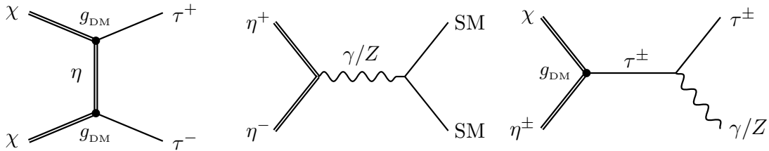
Figure 1. Annihilation and co-annihilation processes.
