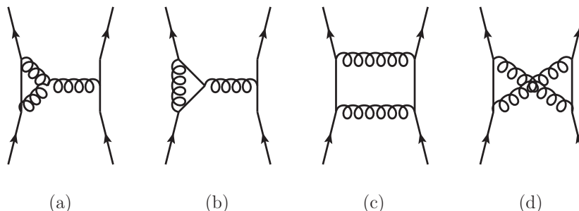
Figure 3. A few sample one-loop diagrams contributing to quark and gluon scattering at next-to-leading order, in the high-energy limit. Diagrams such as (a) and (b) have the same colour structure of the tree-level diagram, and contribute to the one-Reggeon impact factor. Diagrams such as (c) and (d) introduce colour structures different from the colour structure of the tree-level amplitude, and contribute to the two-Reggeon exchange.
