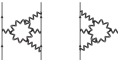
Figure 7. Diagrams representing the colour structure of the 1 \rightarrow 3 and 3 \rightarrow 1 transitions. Notice that these diagrams are different from the ones representing the kinematical structure of the 1 \rightarrow 3 and 3 \rightarrow 1 transitions, i.e. H_{13}(p_1, p_2, p_3) in eq. (3.17). This is a consequence of the fact that the BFKL evolution derived in section 3.1 represents an effective field theory in 2 - 2\epsilon dimensions, in which the longitudinal degrees of freedom have been integrated out.
