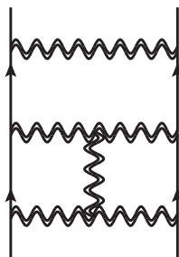
Figure 6. Example of a diagram involved in the calculation of the three-Reggeon cut at three loops. This diagram, together with all the other diagrams obtained by inserting a rung in all possible ways between the three Reggeons, and considering all possible permutation of the three Reggeons themselves, arises from the insertion of a single factor of \hat{H}_{3 \rightarrow 3} , as discussed below eq. (3.42).
