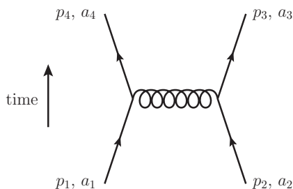
Figure 2. Tree-level t -channel exchange contributing in the high-energy limit to quark-quark, quark-gluon or gluon-gluon scattering. The solid external lines represent either quarks or gluons, depending on the process considered.
