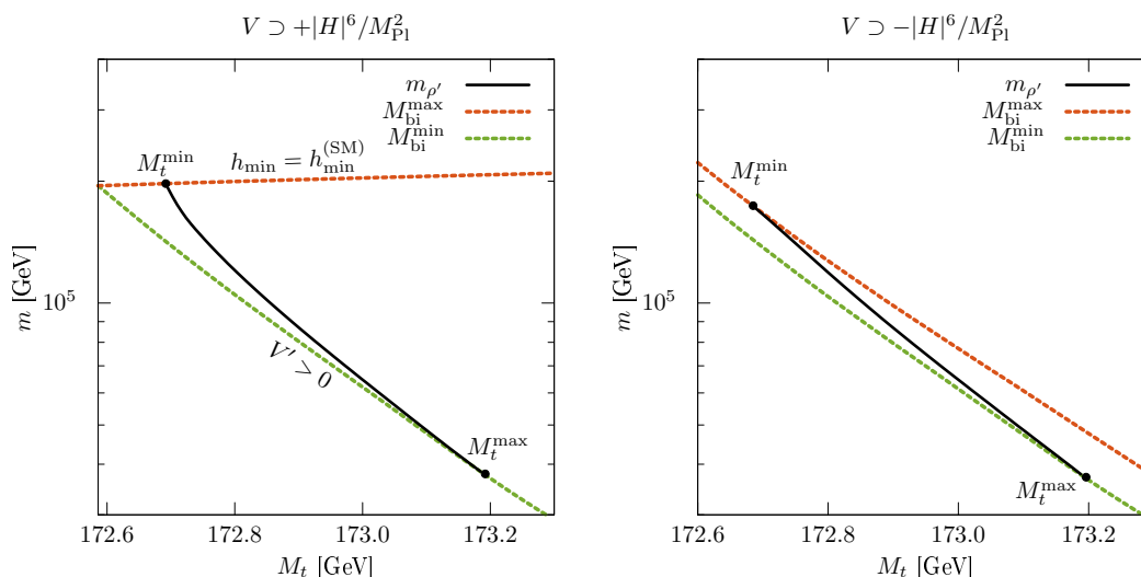
Figure 5. Prediction of m_{\rho'} and viable range of M_t in the presence of Planck-suppressed operators \pm|H|^6/M_{P1}^2 . The minimum and maximum values of the bifundamental scale are defined in the text.
