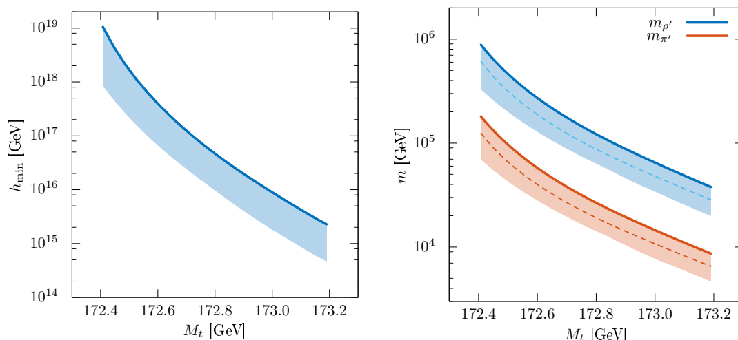
Figure 2. (Left) Dependence of the mirror Higgs VEV on the top quark mass M_t . (Right) The mass of the color octet \rho' (upper line) and \pi' mesons (lower line) as a function of M_t . The uncertainty bands shown are generated by varying the matching scale associated with running the QCD coupling through the strongly coupled regime of QCD'. The solid (dashed) line in each band corresponds to using the four (one) loop QCD' beta function to determine the confinement scale \Lambda_{\text{QCD}'} . Below the lower range of M_t shown the mirror Higgs vev moves above the Planck scale, while above the highest M_t shown no self-consistent solution for bifundamental mass scale exists.
