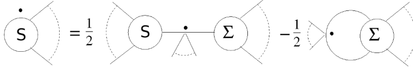
Figure 2. Diagrammatic illustration of a gauge invariant flow equation for gauge fields.
