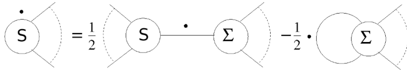
Figure 1. Diagrammatic illustration of a generalised flow equation for scalar fields.
