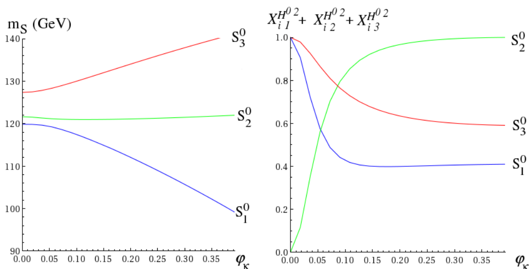
Figure 8. Masses and CP-even composition (X_{i1}^{H^0 2} + X_{i2}^{H^0 2} + X_{i3}^{H^0 2}) for the three lightest Higgs states in the scenario of section 4.1.1 of [94].
