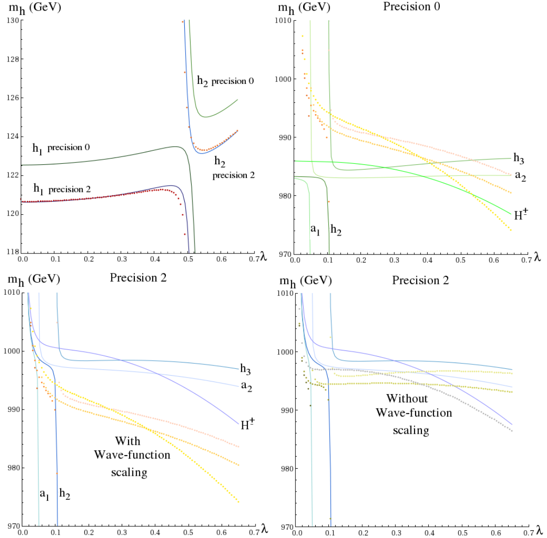
Figure 2. Details on the Higgs masses of figure 1. On the upper left-hand quadrant, we show the Higgs masses close to \sim 125 GeV for precision 0 (green lines), precision 2 (blue lines) and for our implementations (red dots). The plot on the upper right-hand side compares our results (dots) for the ‘heavy’ masses with those of precision 0 (green lines). The same exercise is carried out in the lower left-hand corner for precision 2 (blue lines). In the lower right-hand quadrant, we alter our implementation of the Higgs mass corrections so that all p^2 -dependent terms are taken into account as pole-corrections only (so that the wave-scaling factors are set to 1): the results are displayed as khaki dots and compared to the masses obtained in the procedure of precision 2.
