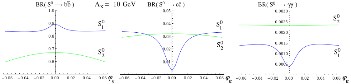
Figure 6. Branching ratios of the light Higgs states for A_\kappa = 10 GeV in the scan of figure 5.
