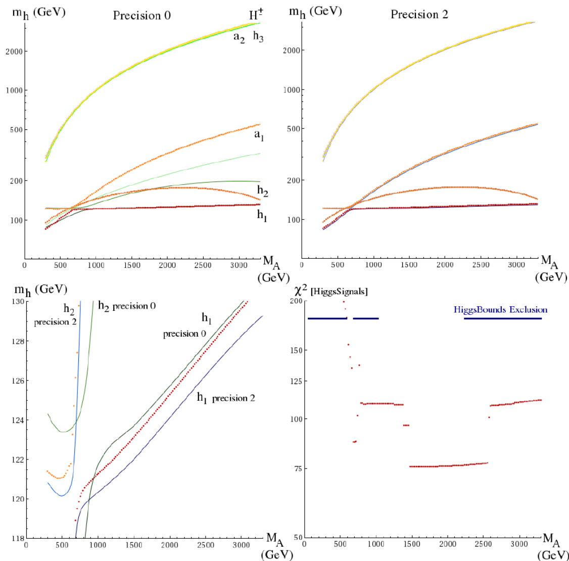
Figure 3. Higgs spectrum for \lambda = 0.7 , \kappa = 0.1 , \tan\beta = 2 , M_A \simeq 2.33\mu_{\text{eff}} + 20.45 \text{ GeV} , M_A \in [0.3, 3] \text{ TeV} , A_\kappa = -50 \text{ GeV} , m_{\tilde{T},\tilde{B}} = 0.5 \text{ TeV} , m_{\tilde{U},\tilde{D}} = 1.5 \text{ TeV} , m_{\tilde{L},\tilde{E}} = 110 \text{ GeV} , 2M_1 = M_2 = 150 \text{ GeV} , M_3 = 1.5 \text{ TeV} , A_{t,b,\tau} = -0.1 \text{ TeV} . Comparison of our results (dots) with precision 0 (upper left-hand plot), precision 2 (upper right-hand plot). Focus on the masses close to 125 GeV (bottom left-hand plot). Finally, results obtained with HiggsBounds and HiggsSignals.
