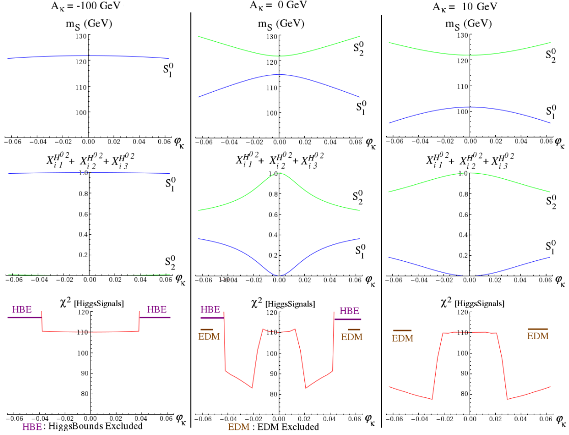
Figure 5. Characteristics of the light Higgs states for \lambda = 0.68 , \kappa = 0.1 , \tan \beta = 2 , \mu_{\text{eff}} = 635 GeV, M_A = 1.5 TeV, A_\kappa = -100, 0, 10 GeV, m_{\tilde{T}, \tilde{B}, \tilde{\tau}} = 0.5 TeV, m_{\tilde{U}, \tilde{D}, \tilde{E}} = 1.5 TeV, 2M_1 = M_2 = M_3/3 = 0.5 TeV, A_{t,b,\tau} = -0.1 TeV. The plots on the first line show how the masses of the Higgs states close to \sim 125 GeV vary with \varphi_\kappa ; the second line displays the magnitude of the scalar components of these states. Characteristics of the lightest state are shown in blue and those for the second lightest are shown in green. Finally, the lower series of plots shows how the points compare to phenomenological limits: the violet mark indicates that the points are excluded by the test in HiggsBounds while the brown mark stands for tensions with the EDM's. The \chi^2 -test of the Higgs data is obtained with HiggsSignals and corresponds to the red curve.
