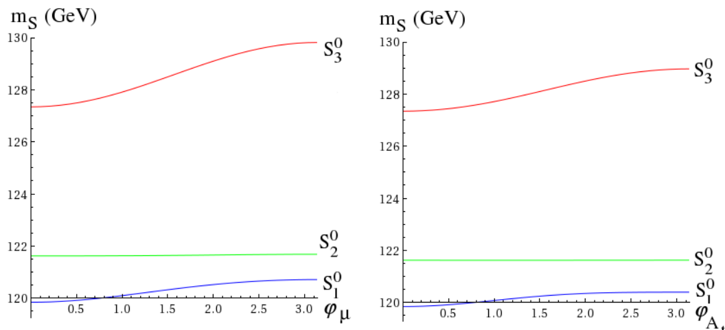
Figure 9. Masses in the scenarios of section 4.1.2 (scan over \varphi_\mu \equiv \varphi_\lambda = \varphi_\kappa ) and section 4.1.3 (scan over \varphi_{A_t} ) of [94].
