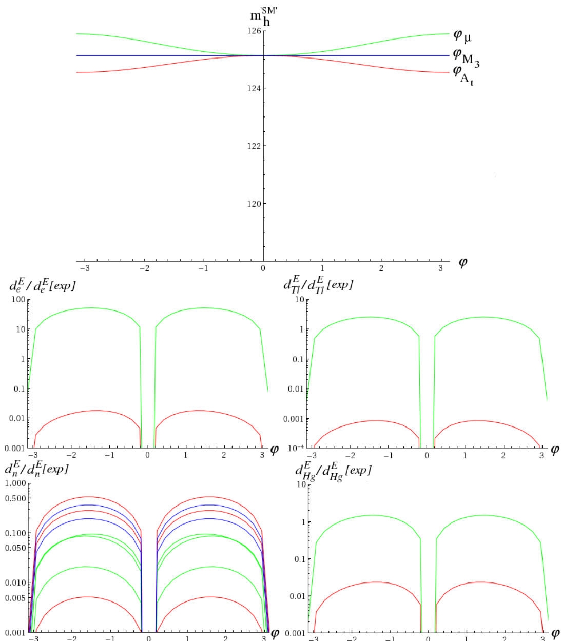
Figure 7. Top: phase-dependence of the mostly h_u^0 Higgs state as obtained from section 4.1 of [89]. Below: estimates of the EDM's (normalized to their experimental upper bounds: see text). The color coding follows that of figure 6 of [89]: green for a scan over \varphi_\mu \equiv \varphi_\lambda = \varphi_\kappa , red for a scan over \varphi_{A_t} and blue for a scan over \varphi_{M_3} . When the blue curve does not appear, the reason is that associated values are negligibly small. Note that several estimates are employed for the neutron EDM.
