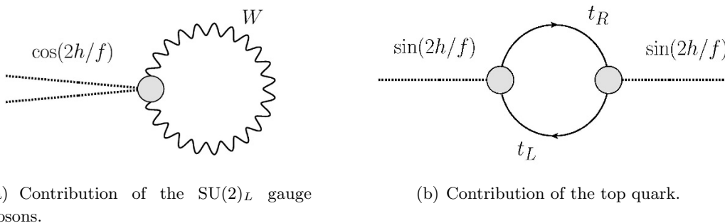
Figure 3. The leading order contributions to the induced Higgs potential.
