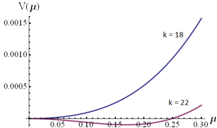
Figure 1. Plot of the potential V(\mu) in units \Lambda = 1 for k = 18 and k = 22 . The transition occurs at k_{\min} \approx 20 . For k > k_{\max} \approx 64 , the minimum is at a value comparable to the cutoff and the approximation breaks down.
