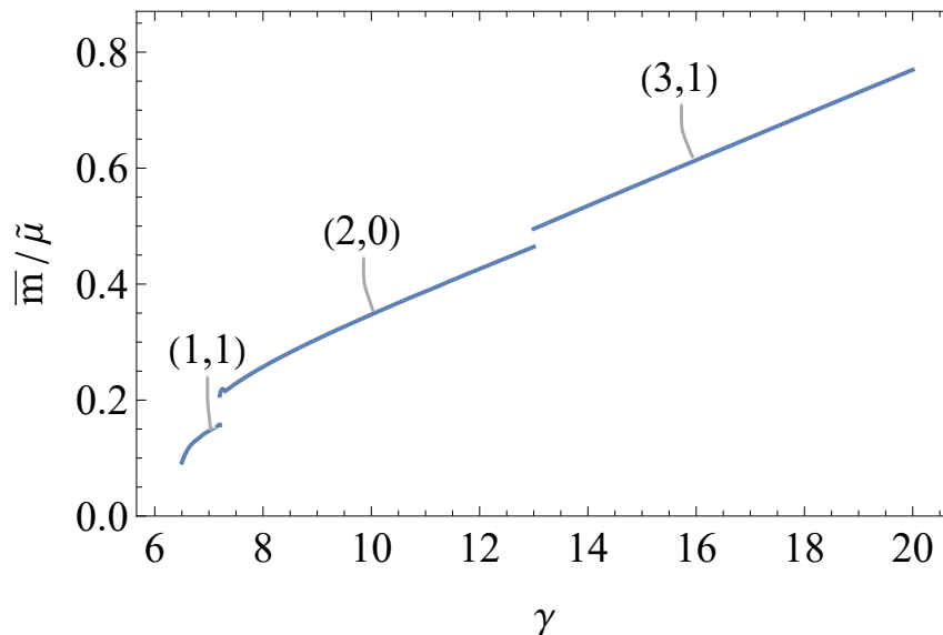
Figure 4. Magnetic moment density averaged over lattice period of alternating ground states.
