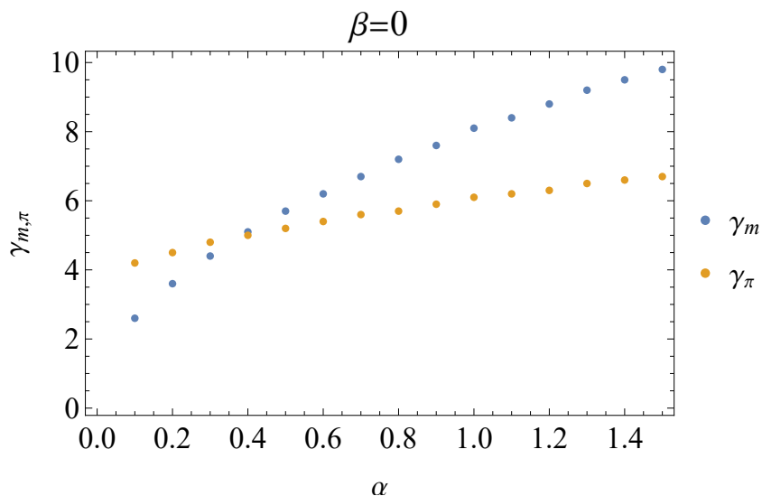
Figure 2. Critical \gamma_{m,\pi} at \beta = 0 and varied \alpha .
