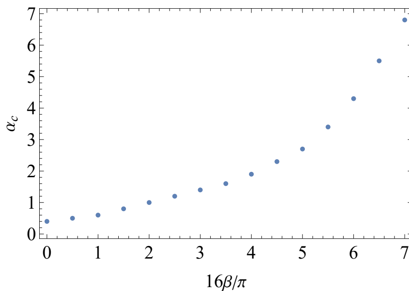
Figure 3. Critical (\alpha_c, \beta) for the ground state to be the mixed soliton lattice. The dots split the \alpha - \beta plane into two regions. In the upper region above the \alpha_c(\beta) , we have \gamma_m < \gamma_\pi .
