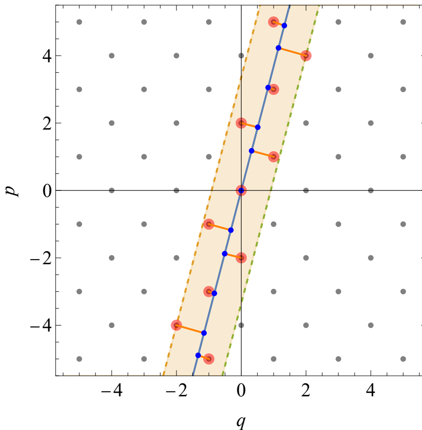
Figure 6. Ground state quasicrystal demonstrated on the p - q plane. Gray dots represent legitimate mixed soliton lattice satisfying eq. (3.2). The blue line has a slope 3/\alpha with \alpha = 0.3e . The light orange band bounded by orange and green dash lines indicates nearby (p, q) dots. These dots are highlighted with burnt orange color. The solid orange lines mark the distances between the (p, q) dots and the p = 3q/\alpha slope. The closer such distance is, the more approximate the (p, q) configuration is to the ground state.
