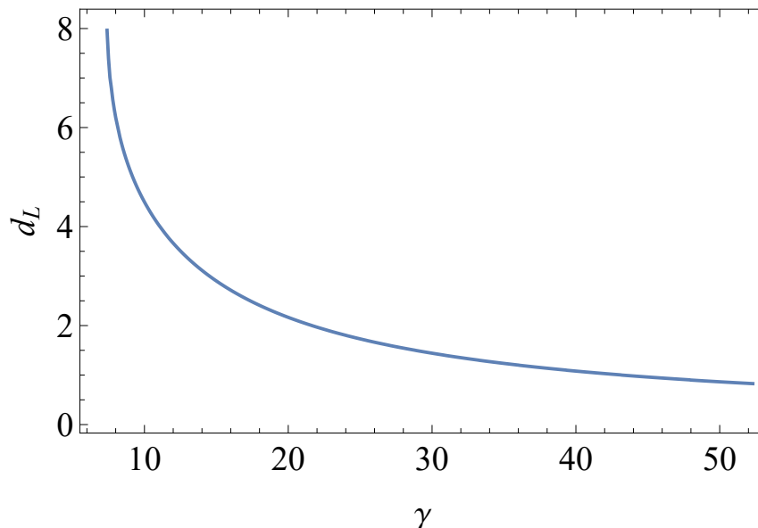
Figure 5. Dependence of the lattice period of configuration (p, q) = (3, 1) on \gamma .
