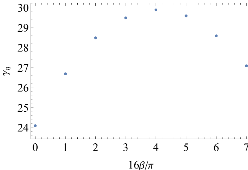
Figure 1. Critical \gamma for \eta' soliton lattice.
