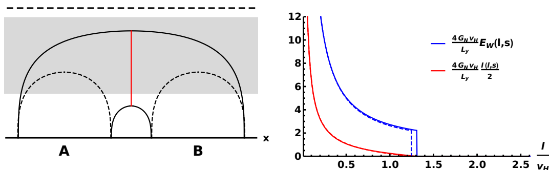
Figure 4. Left: minimal surfaces in the parallel strip case for the electron cloud geometry with T/\mu = 0.02 . The disconnected phase of S(AB) corresponds to the union of the dashed curves. The connected, I(A, B) > 0 , phase on the other hand corresponds to the solid black curves. The dashed black line on the top denotes the black hole horizon while the gray shaded area marks the location of the cloud. The red vertical line corresponds to the minimal surface whose area computes the entanglement wedge cross section in the connected phase. Right: mutual information and entanglement of purification for a parallel strip configuration with separation s/l = 0.4 , as a function of strip width l . The point where I(A, B) vanishes corresponds to the disconnecting of the entanglement wedge. Thus at this point, mutual information vanishes continuously and the entanglement wedge cross section jumps to zero discontinuously. We also show the results for mutual information and entanglement of purification obtained in the pure RN case (dashed red and blue lines, respectively).
