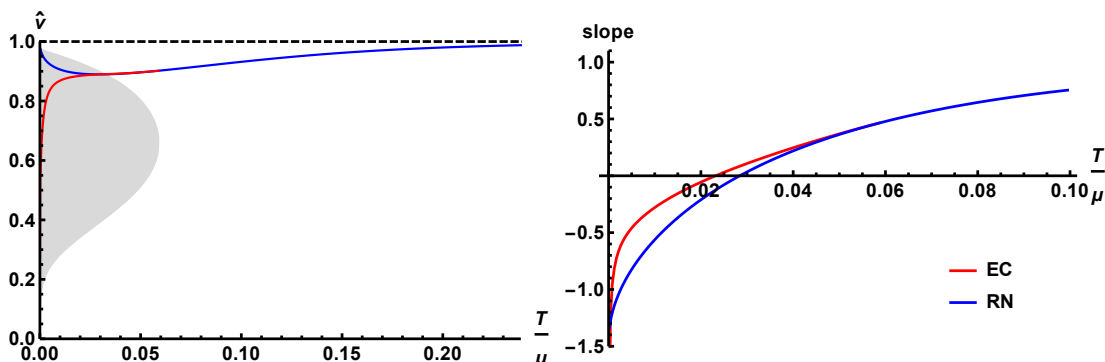
Figure 7. Left: the curves indicate where the shadow region starts in our electron cloud background (red) and in AdS 4 -Reissner-Nordström background (blue). The black dashed line indicates the black hole horizon. The gray area shows the size and position of the bulk charges of the electron cloud. Right: the asymptotic slope of the generalized functional in the limit of large strip width (4.11). In the Reissner-Nordström case, the slope approaches unity at high temperatures because the shadow approaches the event horizon where the weighting function \hat{\gamma}(\hat{v}) vanishes leaving only the area contribution in (4.11).
