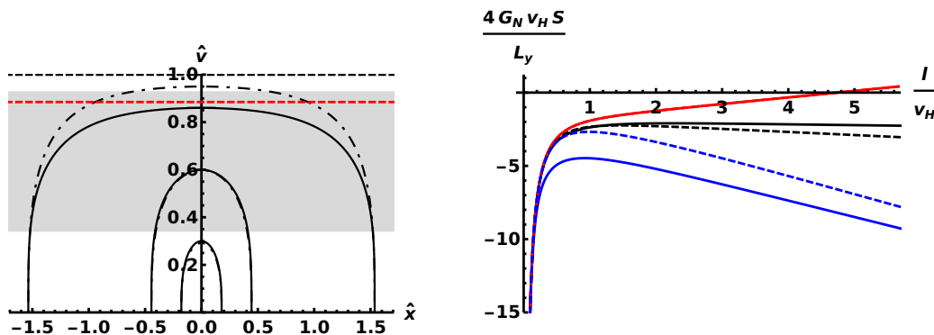
Figure 6. Left: minimal surfaces for a few boundary strips. The solid curves correspond to surfaces which minimize the generalized functional (4.5) while the dash-dotted curves represent RT surfaces of the same boundary strips. It can be seen that the generalized functional is repelled towards the boundary when compared to the corresponding RT surface, but this effect is visible only when the surface penetrates substantially into the cloud (shaded region). The horizontal dashed lines represent the black hole horizon (black) and the edge of the shadow region (red). For this figure we have set T/\mu = 0.02 . Right: the value of the (regularized) generalized functional as a function of strip width. The different curves correspond to T/\mu = 0.0005 (blue), T/\mu = 0.02 (black), and T/\mu = 0.057 (red). We see that strips with small lengths behave similarly for different T/\mu but the long range slope is affected according to the formula (4.11). For comparison, we also show the results for the generalized functional with the same values of T/\mu in the pure RN case (dashed lines).
