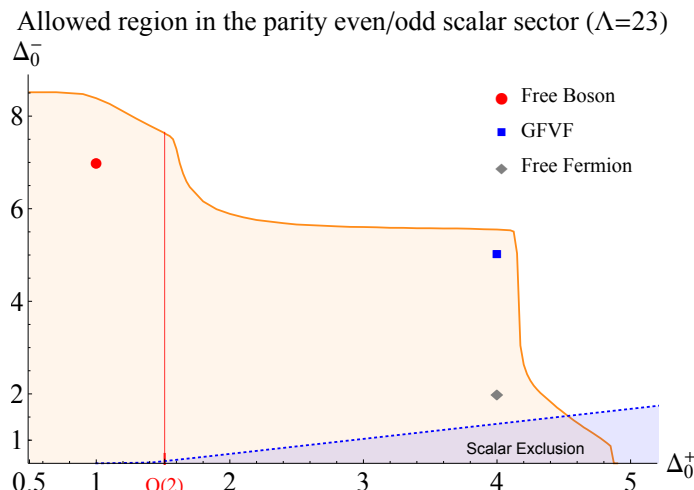
Figure 1. Exclusion plot in the plane (\Delta_0^+, \Delta_0^-) corresponding to the lightest parity even and parity odd scalars appearing in the OPE of two equal conserved currents. The orange shaded region is allowed. The blue region would be excluded by bootstrap constraints on the correlator of four parity odd scalars, see section 3 for details.
