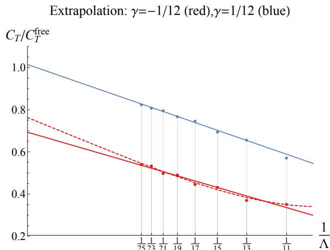
Figure 11. Extrapolation of the bound on central charge normalized to C_T^{\text{free}} as a function of the number of derivatives included in the semidefinite-programming \Lambda . The upper (blue) lines corresponds to a linear fit of the bounds at \gamma = 1/12 . In the limit \Lambda \rightarrow \infty the extrapolation approaches the value 1. The lower curves correspond to a linear (red continuous) and quadratic (red dashed) fit of the bounds at \gamma = -1/12 . The linear fit predicts an asymptotic bound much smaller than the free theory one. Other fits may predict a value of C_T closer to C_T^{\text{free}} . This is exemplified by the quadratic fit.
