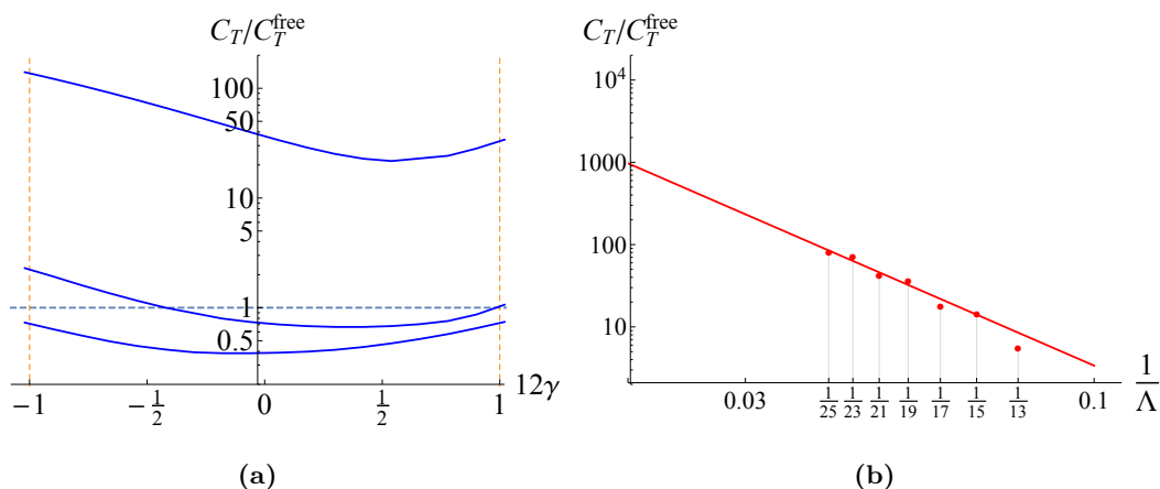
Figure 15. a) Central charge bound as a function of \gamma for several values of the gap in the spin-4 parity even sector, \Delta_4^+ = 5.25, 5.5, 6 . As we increase the gap, solutions consistent with crossing symmetry must develop a larger central charge. b) Extrapolation of the bound on C_T for \gamma = 0, \Delta_4^+ = 6 . Both axis are in logarithmic scale. Linear fit shown as a solid red line suggests that the bound on C_T diverges as \Lambda \rightarrow \infty .
