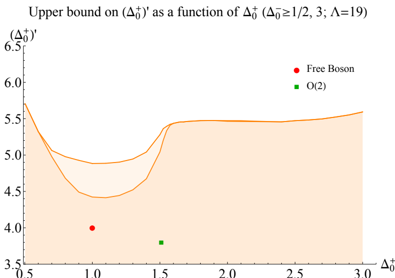
Figure 8. Upper bound on (\Delta_0^+)', the dimension of the second lowest parity-even scalar operator appearing in the OPE J \times J when we assume that the theory contains a scalar parity-even operator with dimension \Delta_0^+. The red dot corresponds to the free boson ((\Delta_0^+, (\Delta_0^+)') = (1, 4)), and green dot corresponds to interacting O(2) theory, while points for the free fermion and GFVF lie outside the range of the plot. Lower curve assumes theory has no relevant scalar parity-odd operators. The bounds have been computed with \Lambda = 19.
