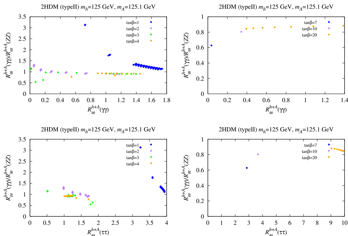
Figure 8. Correlations between R_{gg}^{h+A}(\gamma\gamma)/R_{gg}^{h+A}(ZZ) and R_{gg}^{h+A}(\gamma\gamma) (upper panels) and R_{gg}^{h+A}(\tau\tau) (lower panels) for selected values of \tan\beta .
