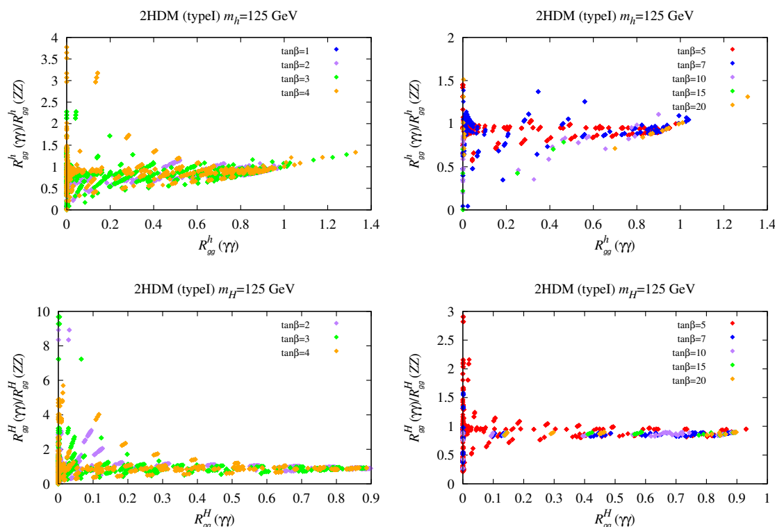
Figure 4. For the h (top) and H (bottom) we plot the gluon fusion induced \gamma\gamma/ZZ ratio as a function of R_{gg}(\gamma\gamma) for the Type I 2HDM1.
