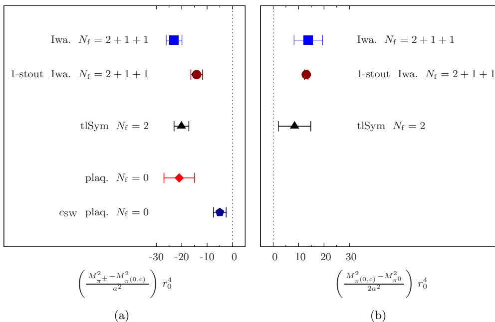
Figure 5. Comparison of the values of the mass-splittings (a) (M_{\pi^\pm}^2 - M_{\pi^{(0,c)}}^2)/a^2 and (b) (M_{\pi^{(0,c)}}^2 - M_{\pi^0}^2)/2a^2 from different lattice setups (see text for details).
