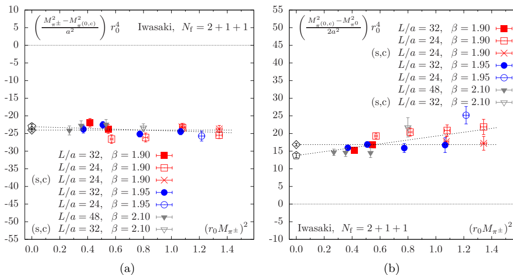
Figure 1. Determination of the mass-splittings (a) (M_{\pi^{\pm}}^2 - M_{\pi^{\pm}}^2(0,c))/a^2 in eq. (2.6) and (b) (M_{\pi^{\pm}}^2(0,c) - M_{\pi^{\pm}}^2)/2a^2 in eq. (2.7) as a function of M_{\pi^{\pm}}^2 . These quantities are in units of the chirally extrapolated Sommer scale r_0 . The mass-splittings are directly related to the Wilson LECs W'_8 and W'_6 . The lattice setup with the Iwasaki gauge action and N_f = 2 + 1 + 1 flavours of Wilson twisted mass fermions is considered. Filled and empty symbols signal a change in the lattice size. The label “(s,c)” in the legend indicates the effect of changing the values of the strange and charm quark masses in the sea. The mass-splittings illustrated in these figures assess the size of O(a^2) discretisation effects. Hence, any lattice spacing dependence in these quantities points to residual higher order discretisation effects. The results of a chiral extrapolation from a constant and a linear fit in M_{\pi^{\pm}}^2 are shown. The deviation between the two extrapolated values is included in the systematic error analysis.
