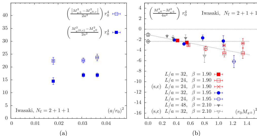
Figure 2. (a) Lattice spacing dependence of the mass-splittings |M_{\pi^\pm}^2 - M_{\pi^{(0,c)}}^2|/a^2 — empty symbols — and (M_{\pi^{(0,c)}}^2 - M_{\pi^0}^2)/2a^2 — filled symbols — at a reference mass (M_{\pi^\pm} r_0)^2 \approx 0.55 . For a better visibility, the absolute value of the mass splitting is considered in the case of the empty symbols. (b) Pion mass-splitting, (M_{\pi^0}^2 - M_{\pi^\pm}^2)/a^2 , normalised according to eq. (2.9) in order to relate it to the combination of Wilson LECs c_2 . The chiral extrapolation using a constant and a linear fit in M_{\pi^\pm}^2 is also shown. The lattice setup with the Iwasaki gauge action and N_f = 2 + 1 + 1 flavours of Wilson twisted mass fermions is considered.
