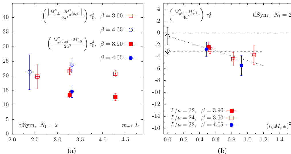
Figure 4. (a) Finite volume effects on the mass-splittings |M_{\pi^\pm}^2 - M_{\pi^{(0,c)}}^2|/a^2 — empty symbols — and (M_{\pi^{(0,c)}}^2 - M_{\pi^0}^2)/2a^2 — filled symbols. Note that the absolute value of the mass-splitting is used in the case of empty symbols. (b) Pion mass-splitting, (M_{\pi^0}^2 - M_{\pi^\pm}^2)/a^2 , normalised according to eq. (2.9) in order to relate it to the combination of Wilson LECs c_2 . The chiral extrapolation using a constant and a linear fit in M_{\pi^\pm}^2 is also shown. The lattice setup with the tree-level Symanzik improved (tlSym) gauge action and N_f = 2 flavours of Wilson twisted mass fermions is considered.
