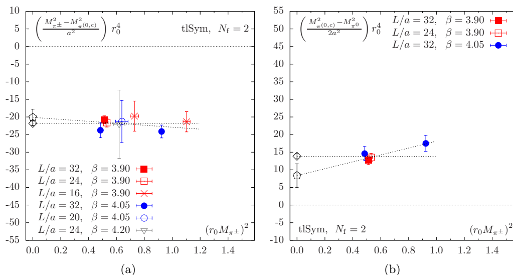
Figure 3. Determination of the mass-splittings (a) (M_{\pi^\pm}^2 - M_{\pi^{(0,c)}}^2)/a^2 in eq. (2.6) and (b) (M_{\pi^{(0,c)}}^2 - M_{\pi^0}^2)/2a^2 in eq. (2.7) as a function of M_{\pi^\pm}^2 . These quantities are in units of the chirally extrapolated Sommer scale r_0 . The mass-splittings are directly related to the Wilson LECs W'_8 and W'_6 . The lattice setup with the tree-level Symanzik improved (tlSym) gauge action and N_f = 2 flavours of Wilson twisted mass fermions is considered. Filled and empty symbols signal a change in the lattice size.
