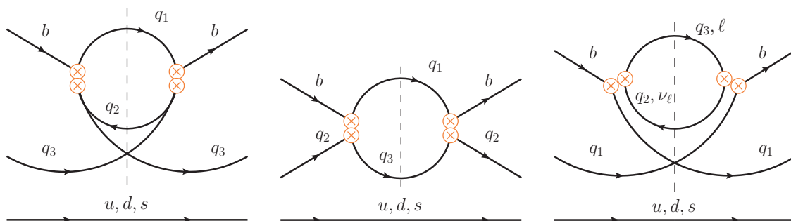
Figure 2. Diagrams corresponding, from left to right, to the \text{int}^- , \text{exc} , and \text{int}^+ topologies at LO-QCD. The numbering scheme for quarks follows that in eq. (2.3), so that q_{1,2} are up-type quarks and q_3 is down-type. Note that semileptonic contributions only arise in the \text{int}^+ topology. Disregarding the second, non-interacting spectator quark, these topologies are related by crossing to those in meson decays, cf. footnote 7.
