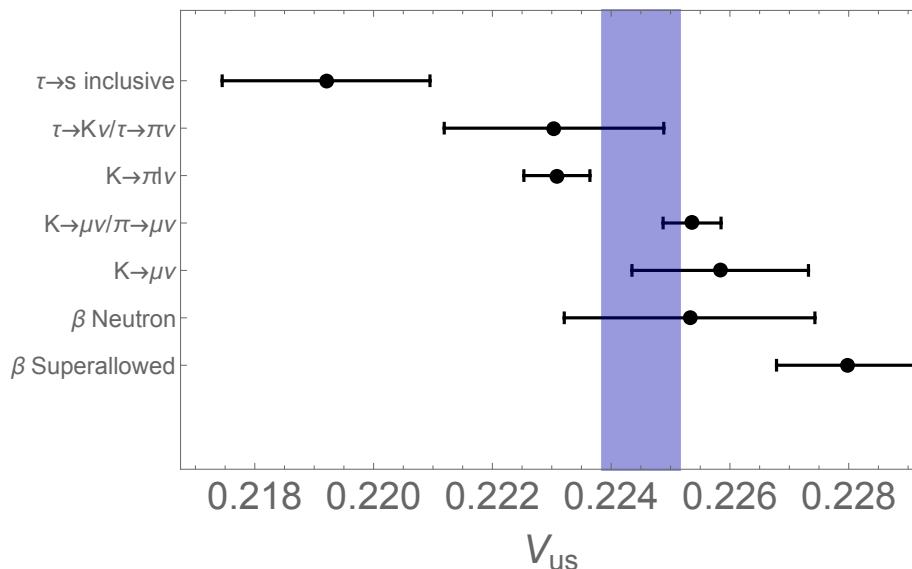
Figure 5. 68% CL constraints on the Cabibbo angle assuming the SM is the UV completion of our EFT, which implies \epsilon_X^{D\ell} = 0 . We show the separate constraints from the most precise measurement probing this parameter: inclusive \tau \rightarrow s decays, 2-body tau decays, semileptonic kaon decay, the ratio \Gamma(\pi \rightarrow \mu\nu_\mu)/\Gamma(K \rightarrow \mu\nu_\mu) , \Gamma(K \rightarrow \mu\nu_\mu) , neutron beta decay, and the superallowed 0^+ \rightarrow 0^+ nuclear beta decays. The purple band corresponds to a combination of these measurements with errors inflated à la PDG with the scale factor of S = 2.0 , so as to account for the large tension between the individual inputs.
