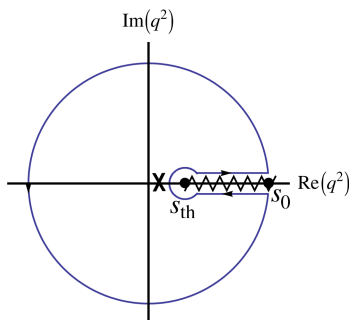
Figure 7. Contour of integration for eq. (A.2).
