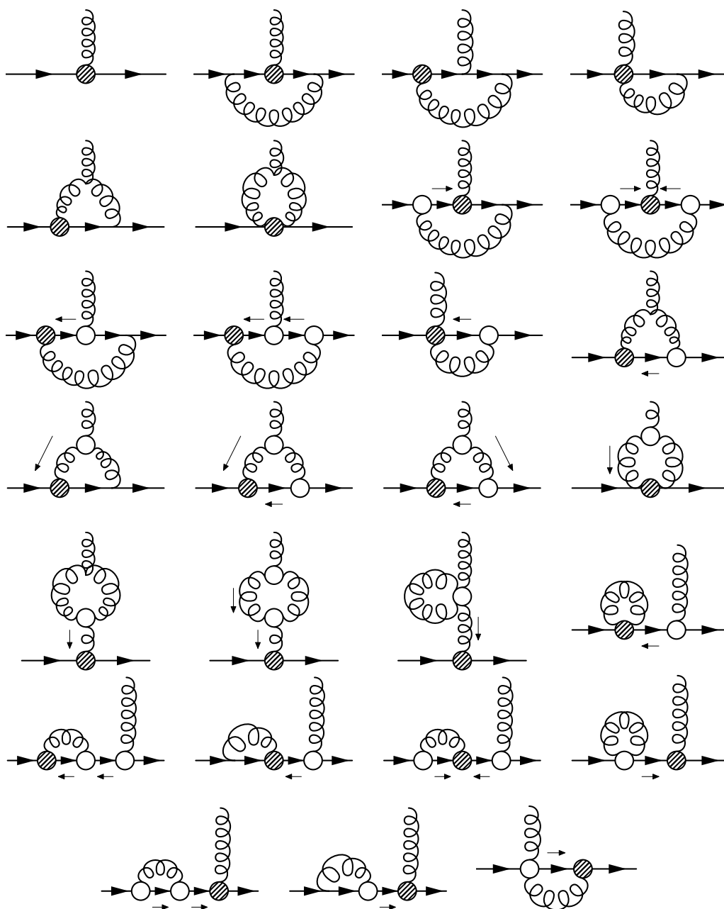
Figure 2. Feynman diagrams for the matching calculation of the flowed qCEDM operator. We do not show 19 additional diagrams that follow from crossing and inverting the fermion-flow direction. The hatched blob denotes the insertion of the flowed qCEDM operator at flow time t , while the open circles are flow vertices. Normal quark and gluon lines denote propagators, while lines with an adjacent arrow stand for flow lines. The adjacent arrow points into the direction of increasing flow time.
