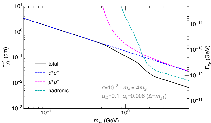
Figure 8. \chi_2 decay length together with the leptonic and the hadronic contributions for the parameters of figure 5 (left).
