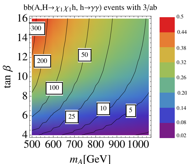
Figure 13. The number of pp \rightarrow b\bar{b}(A, H), (A, H) \rightarrow \chi_1\chi_h, \chi_h \rightarrow \chi_1h, h \rightarrow \gamma\gamma events (summed over A and H ) at the HL-LHC. For this plot, we choose the spectrum \mu = m_A/2 - 10 GeV, M_1 = \mu - 130 GeV, so that A/H \rightarrow \chi_1\chi_h as well as \chi_h \rightarrow \chi_1 + h are kinematically open (for these parameters, we find BR(\chi_h \rightarrow \chi_1h) \approx BR(\chi_h \rightarrow \chi_1Z) , where h represents a sum over 2, 3). The color coding shows the ratio of this production cross section (not including the BR(h \rightarrow \gamma\gamma) ) to the production cross section of mono-h final states from direct electroweakino production, pp \rightarrow \chi_i\chi_j \rightarrow h + \cancel{E}_T .
