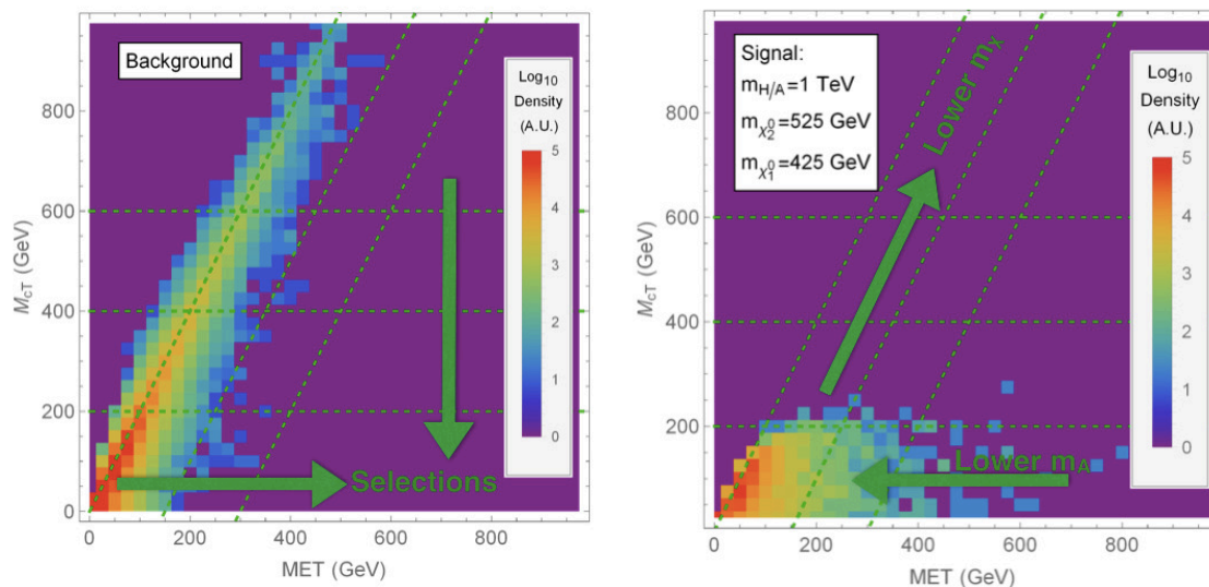
Figure 5. The background (left panel) and signal (right panel) distributions in the \cancel{E}_T - m_{cT}(\ell\ell, \cancel{E}_T) plane. The signal distribution is shown for a representative benchmark point with m_H = m_A = 1 TeV, m_{\chi_1} = 425 GeV, and m_{\chi_2} = 525 GeV. In the left panel, we show with dashed green lines and arrows the direction of the selection grid described in the text. In the right panel, green arrows indicate how the signal distribution shifts as the heavy Higgs or neutralino masses are varied.
