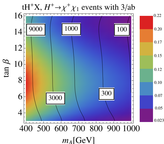
Figure 14. The number of events for pp \rightarrow tH^\pm X, H^\pm \rightarrow \chi^\pm \chi_1 at the HL-LHC. This plot uses the same mass spectrum as of figure 3 (left panel): in particular, M_1 = 150 GeV and \mu = m_A - 175 GeV. The color coding denotes the branching ratio \text{BR}(H^+ \rightarrow \chi^+ \chi_1) .
