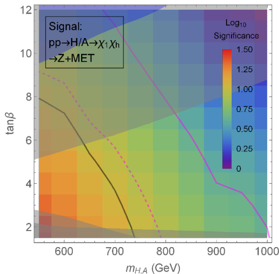
Figure 7. The projected 2\text{-}\sigma exclusion limit (magenta) and 5\text{-}\sigma discovery reach (dashed magenta) for 13 TeV HL-LHC in the m_A\text{-}\tan\beta plane, for fixed m_{\chi_{2,3}} = 300 GeV and m_{\chi_1} = 100 GeV. The solid black curve denotes the corresponding 2\sigma exclusion with 300\text{ fb}^{-1} . The colors on each benchmark point tile represent the projected significance of our analysis at 13 TeV HL-LHC. For comparison, we also show the projected limits at HL-LHC for heavy Higgs searches in the \tau\tau [84] and t\bar{t} [4] final states in the upper shaded and lower shaded regions, respectively. The current constraints from A/H \rightarrow \tau\tau searches [1, 2] are shown in the blue shaded region. The lower shaded region that vanishes around 700 GeV represents possible limits from the 4-top final state, for t\bar{t} associated production of the heavy Higgs ( pp \rightarrow t\bar{t}H/A , H/A \rightarrow t\bar{t} ) (taken from [5]).
