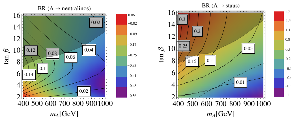
Figure 3. Left panel: curves with numerical labels denote contours of \text{Br}(A \rightarrow \text{neutralinos}) . For this scan, we set M_1 = 150 \text{ GeV} , \mu = m_A - 175 \text{ GeV} , M_2 = 2 \text{ TeV} , all soft terms A_f = \mu / \tan \beta + 1600 \text{ GeV} , and all other dimensionful parameters to 1.5 \text{ TeV} . These parameters are similar to the m_h^{\text{mod}+} scenarios from [59], except for the modified values of M_1 , M_2 , and \mu . The color coding represents the ratio of electroweakino production cross section via heavy Higgs decay to direct Drell-Yan production cross section, \log_{10}(\sigma(pp \rightarrow A, H \rightarrow \text{neutralinos})/\sigma(pp \rightarrow \text{electroweakinos})) , where the numerator includes contributions from both gluon fusion and b -associated production of A and H , and the denominator includes all direct neutralino and chargino production modes. The dashed line indicates the contour along which these two production cross sections are equal. Right panel: analogous plot for \text{Br}(A \rightarrow \text{staus}) , with parameter choices the same as for the neutralino plot, except m_{\tilde{\tau}_L} = m_{\tilde{\tau}_R} = m_A/2 - 50 \text{ GeV} , A_\tau = 1 \text{ TeV} , and \mu = 500 \text{ GeV} , which are similar to the light stau scenario in [59] except for the modified values of A_\tau , m_{\tilde{\tau}_L} , m_{\tilde{\tau}_R} , and M_2 . In both panels, the shaded regions represent the parameter space excluded by current LHC searches for A/H \rightarrow \tau\tau [1, 2], whereas all non-shaded regions are consistent with all current LHC bounds from various searches.
