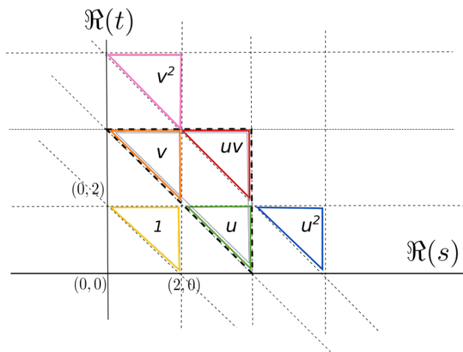
Figure 8. The fundamental domains for the Mellin transform of R\mathcal{H} .
