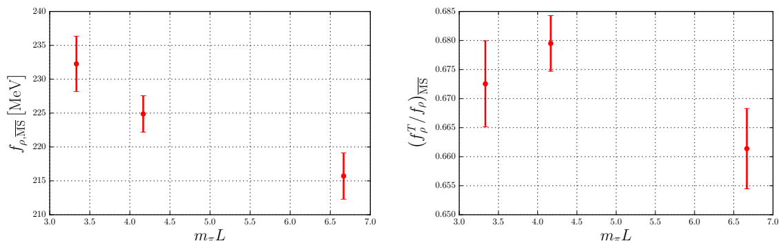
Figure 4. Volume dependence of f_\rho (left panel) and f_\rho^T/f_\rho (right panel) at \beta = 5.29 , \kappa = 0.13632 .
