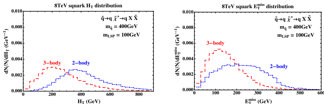
Figure 1. H_T and \cancel{E}_T distributions for squark pair production in the Single-Invisible and Double-Invisible scenarios. In this example, m_{\tilde{q}} = 400 GeV and m_{\text{LSP}} = 100 GeV.
