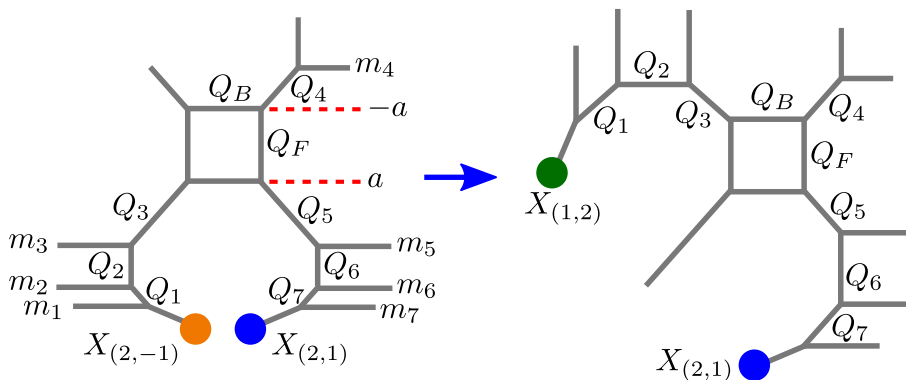
Figure 17. This figure shows the brane configuration for N_f = 7 with two 7-branes. Using the Hanany-Witten effect we obtain a fiber-base invariant configuration.
