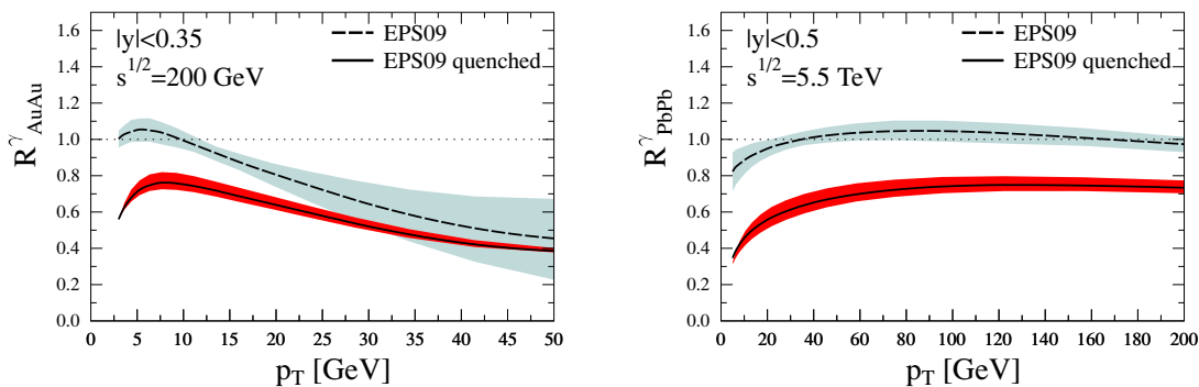
Figure 10. Upper bands: Same as figure 9 using the EPS09 nPDF sets. Lower bands: Nuclear production ratio R_{AA}^\gamma using the central EPS09 nPDF set and after downscaling the fragmentation component by a factor of five. The band corresponds to a scale variation from p_T/2 to 2p_T .
