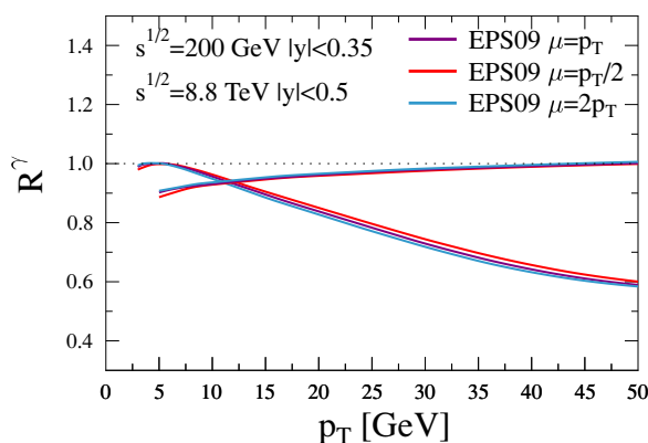
Figure 8. Scale dependence of the nuclear modification ratio R_{dAu}^{\gamma} for mid-rapidity prompt photon production at RHIC (lower curve) and LHC (upper curve). Calculations are performed using the central EPS09 nPDF set and varying all scales by a factor of two with respect to the photon transverse momentum; see the text for details.
