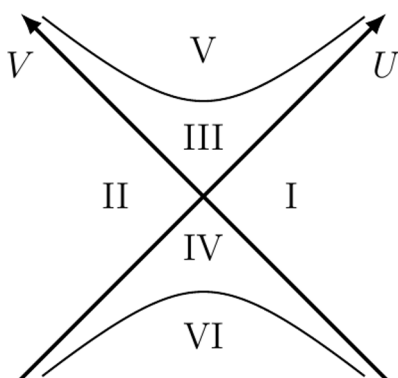
Figure 1. Space-time diagram for the Lorentzian black hole (1.1). The cross defined by the equation UV = 0 is a horizon, while the metric possesses a physical singularity on the hyperbola UV = 1 .
