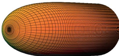
Figure 2. Visualization of the 2D manifold with metric (1.2).
